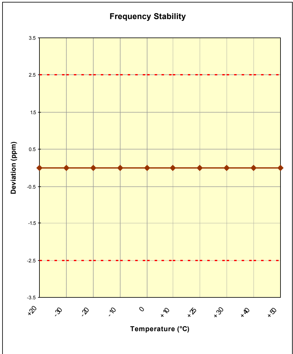
Figure 6-2. Frequency Stability Graph (PCS CDMA Mode – Ch. 600)
