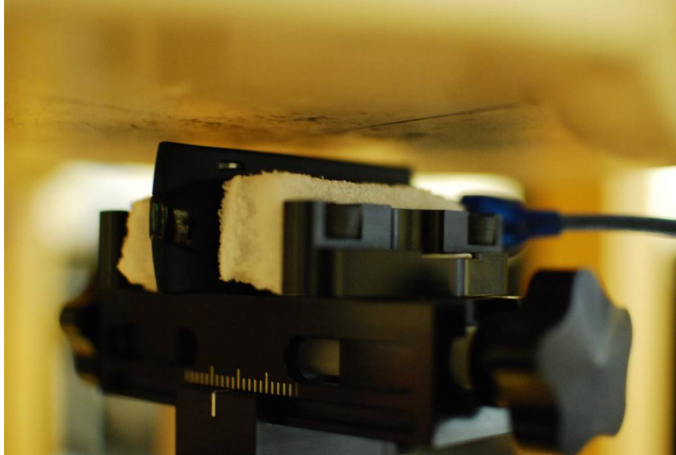
SAR Test Setup Photo 3 – Vertical Front at 0.5 cm
