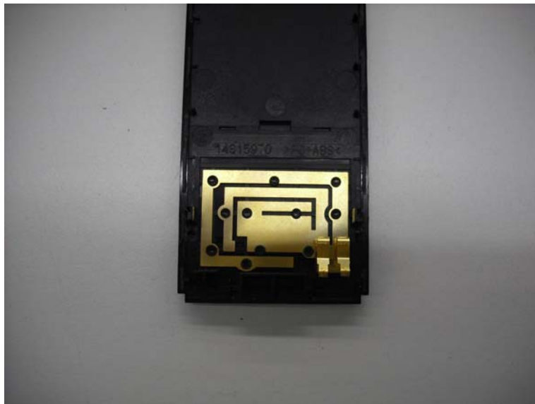
Diversity Antenna Close Up
