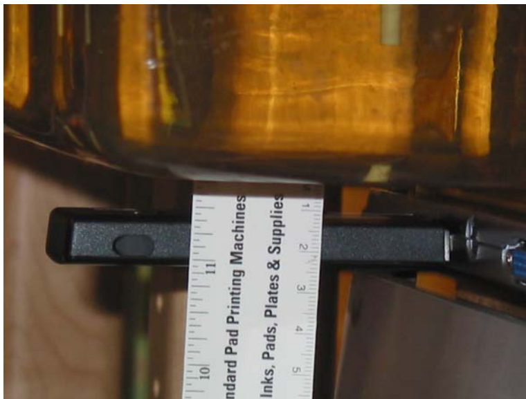
Bottom Installed In Toshiba Laptop
