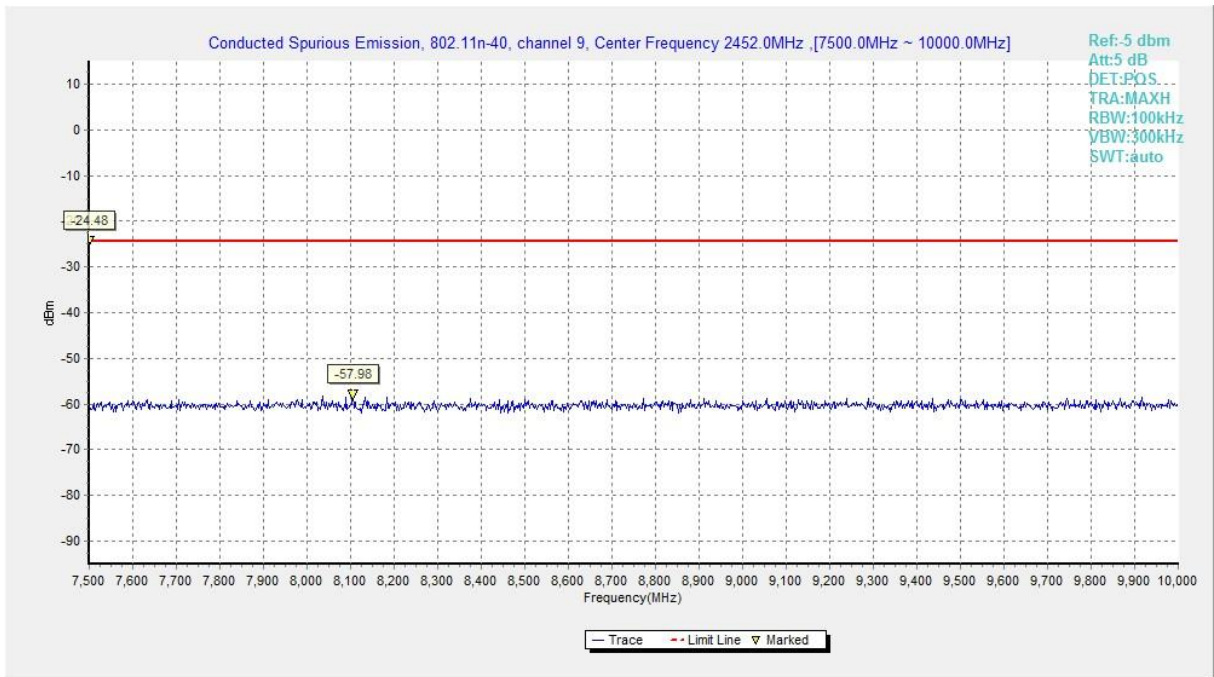
Fig.A.6.1.141 Transmitter Spurious Emission - Conducted (802.11n-HT40, Chain1, Ch9, 7.5 GHz-10 GHz)
