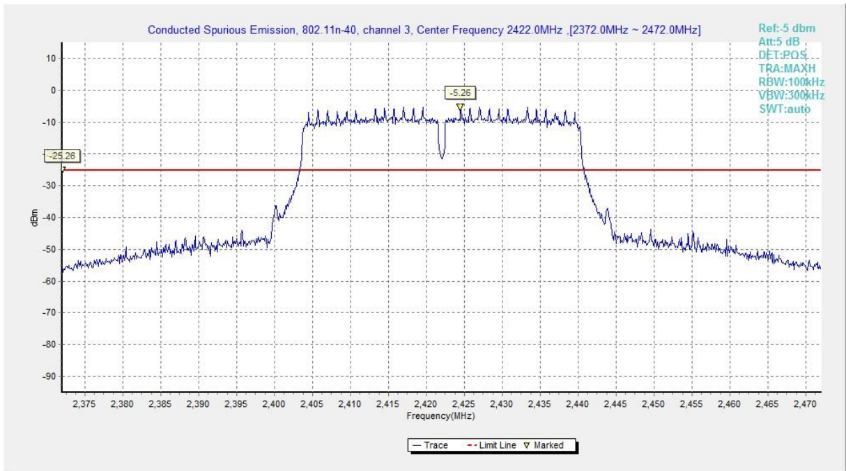
Fig.A.6.1.97 Transmitter Spurious Emission - Conducted (802.11n-HT40, Chain0, Ch3, Center Frequency)
