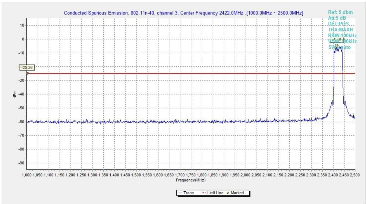
Fig.A.6.1.99 Transmitter Spurious Emission - Conducted (802.11n-HT40, Chain0, Ch3, 1 GHz-2.5 GHz)
