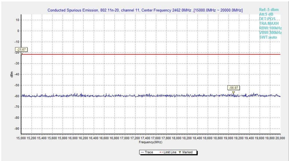
Fig.A.6.1.95 Transmitter Spurious Emission - Conducted (802.11n-HT20, Chain1, Ch11, 15 GHz-20 GHz)
