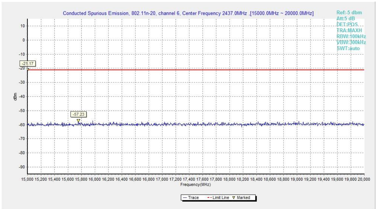
Fig.A.6.1.87 Transmitter Spurious Emission - Conducted (802.11n-HT20, Chain1, Ch6, 15 GHz-20 GHz)
