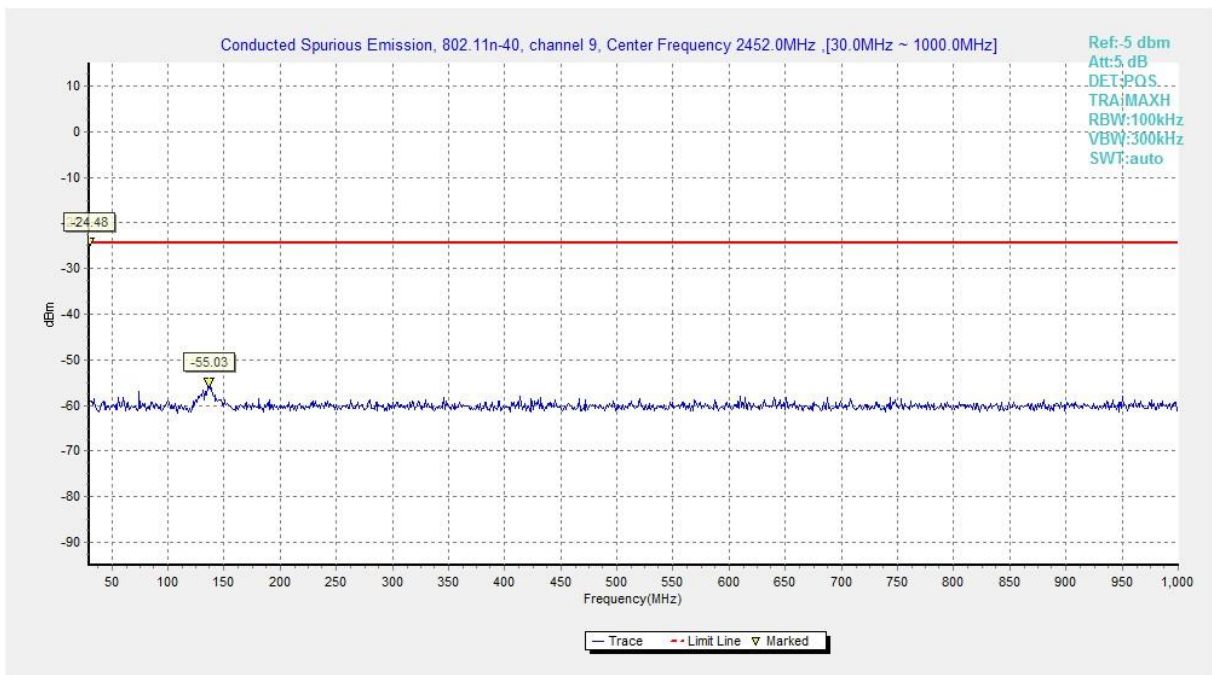
Fig.A.6.1.138 Transmitter Spurious Emission - Conducted (802.11n-HT40, Chain1, Ch9, 30 MHz-1 GHz)
