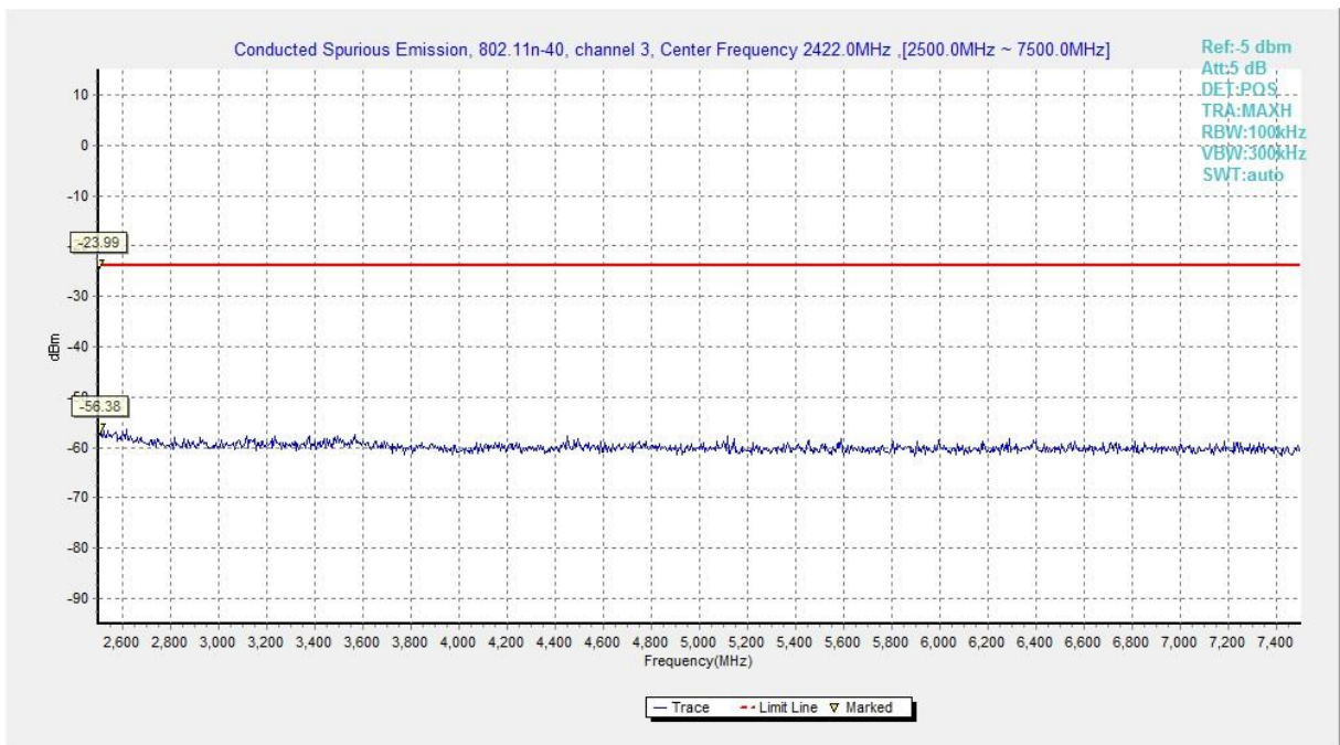
Fig.A.6.1.124 Transmitter Spurious Emission - Conducted (802.11n-HT40, Chain1, Ch3, 2.5 GHz-7.5 GHz)
