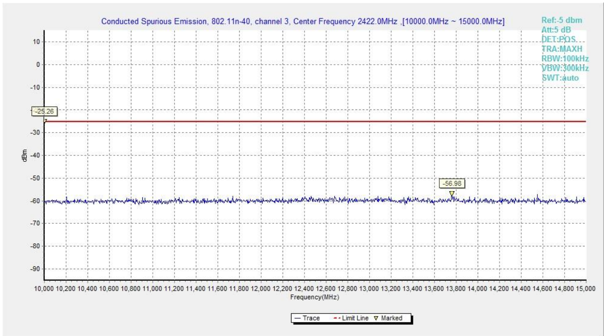
Fig.A.6.1.102 Transmitter Spurious Emission - Conducted (802.11n-HT40, Chain0, Ch3, 10 GHz-15 GHz)
