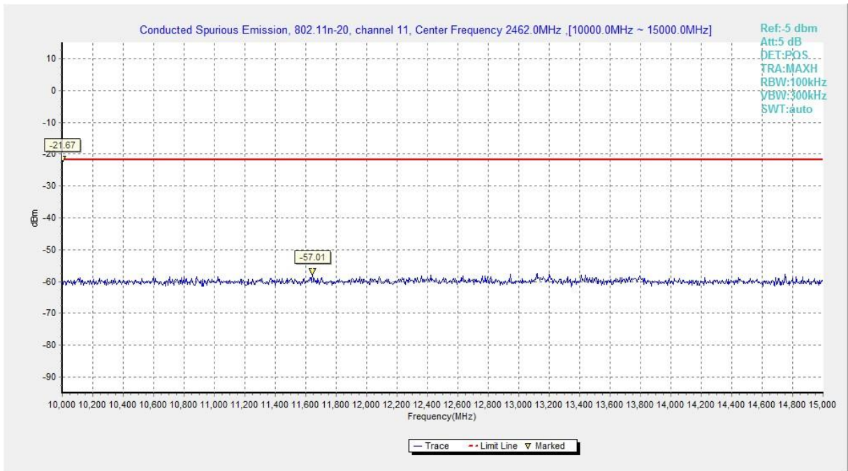
Fig.A.6.1.94 Transmitter Spurious Emission - Conducted (802.11n-HT20, Chain1, Ch11, 10 GHz-15 GHz)
