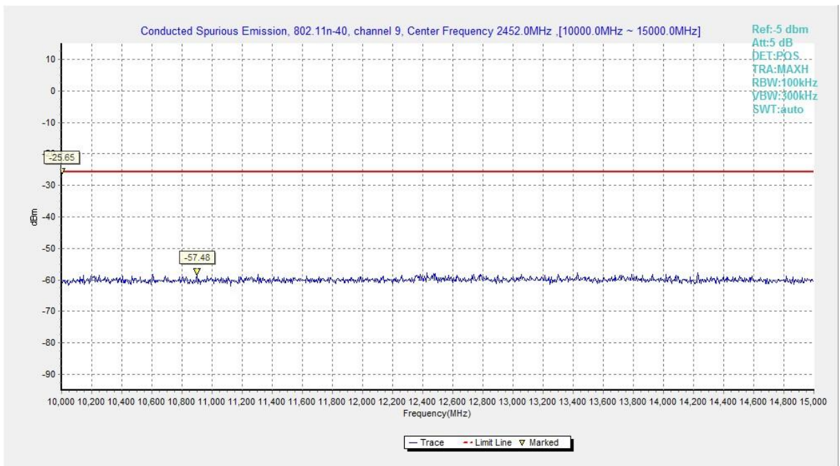
Fig.A.6.1.118 Transmitter Spurious Emission - Conducted (802.11n-HT40, Chain0, Ch9, 10 GHz-15 GHz)
