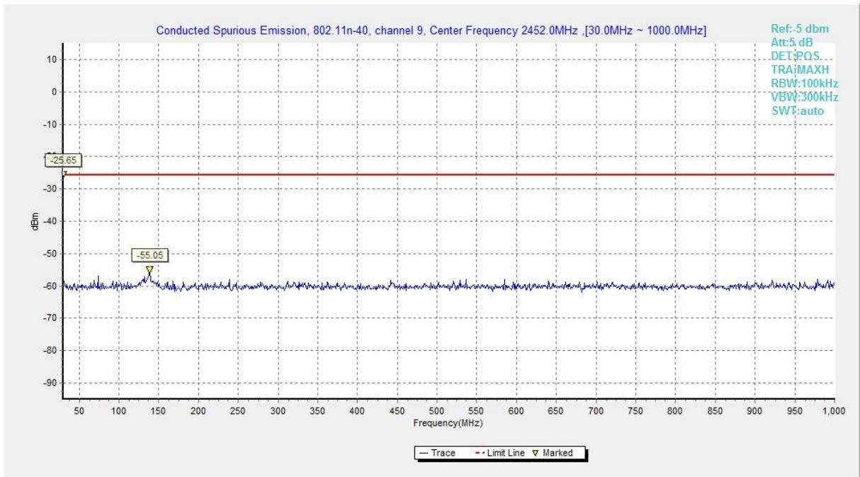
Fig.A.6.1.114 Transmitter Spurious Emission - Conducted (802.11n-HT40, Chain0, Ch9, 30 MHz-1 GHz)
