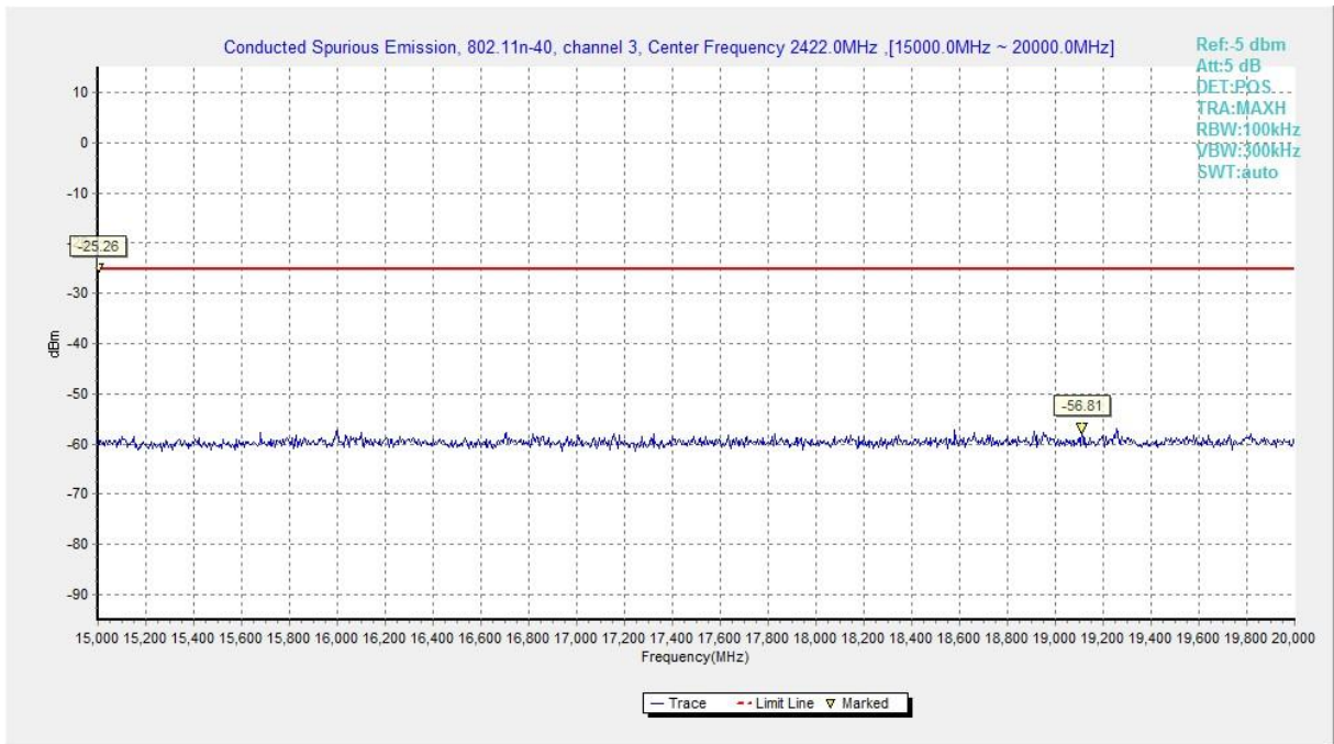
Fig.A.6.1.103 Transmitter Spurious Emission - Conducted (802.11n-HT40, Chain0, Ch3, 15 GHz-20 GHz)
