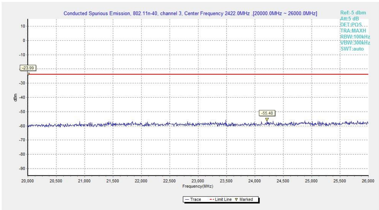
Fig.A.6.1.128 Transmitter Spurious Emission - Conducted (802.11n-HT40, Chain1, Ch3, 20 GHz-26 GHz)
