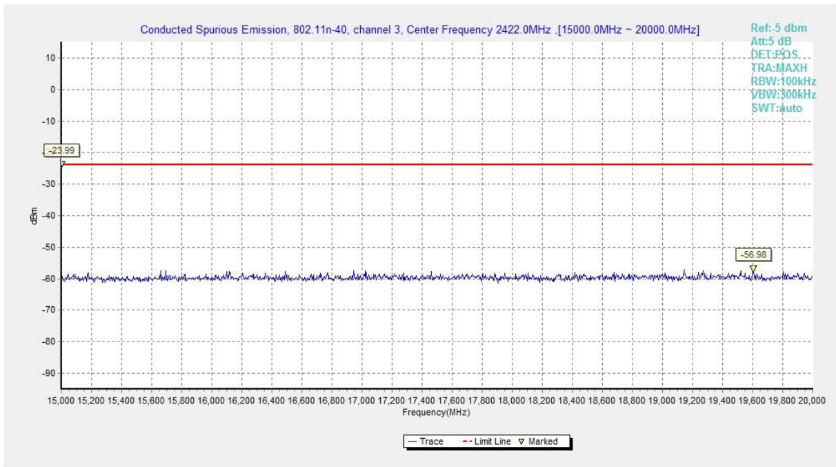
Fig.A.6.1.127 Transmitter Spurious Emission - Conducted (802.11n-HT40, Chain1, Ch3, 15 GHz-20 GHz)
