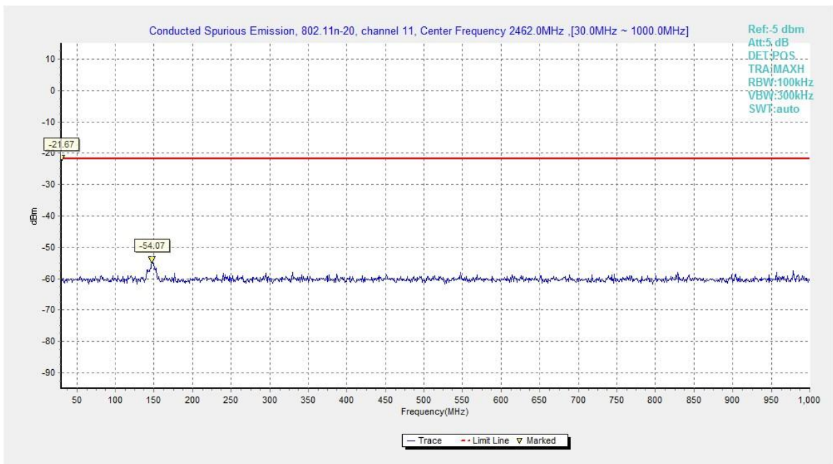
Fig.A.6.1.90 Transmitter Spurious Emission - Conducted (802.11n-HT20, Chain1, Ch11, 30 MHz-1 GHz)
