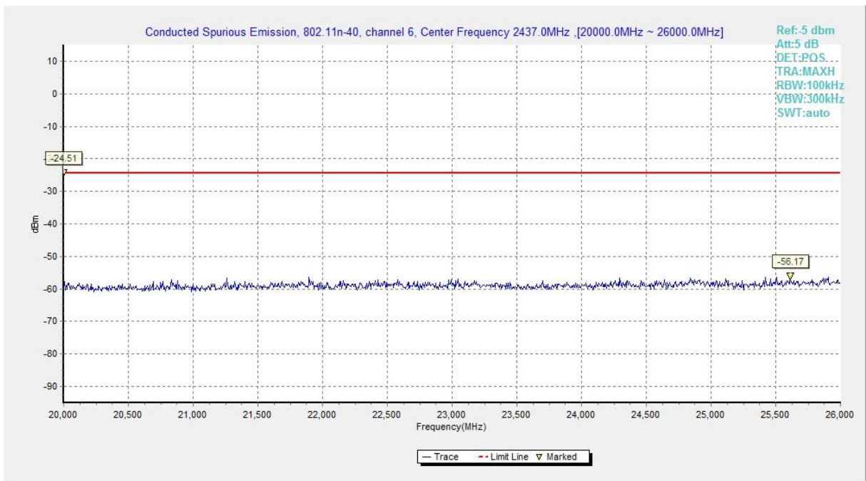
Fig.A.6.1.136 Transmitter Spurious Emission - Conducted (802.11n-HT40, Chain1, Ch6, 20 GHz-26 GHz)
