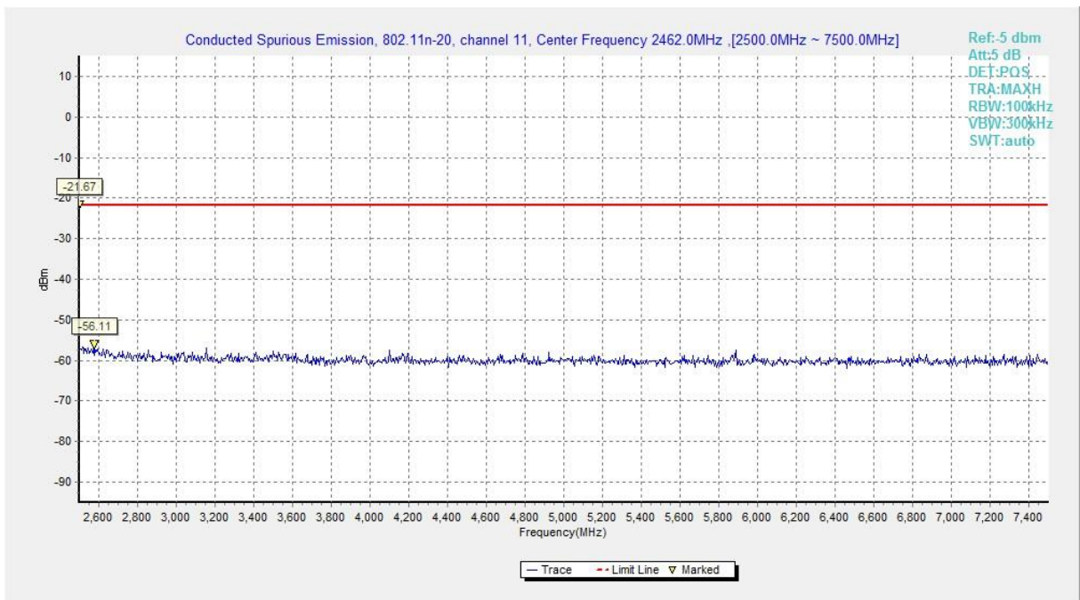
Fig.A.6.1.92 Transmitter Spurious Emission - Conducted (802.11n-HT20, Chain1, Ch11, 2.5 GHz-7.5 GHz)
