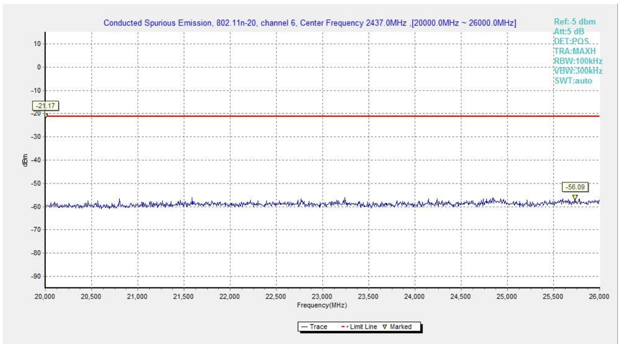
Fig.A.6.1.88 Transmitter Spurious Emission - Conducted (802.11n-HT20, Chain1, Ch6, 20 GHz-26 GHz)
