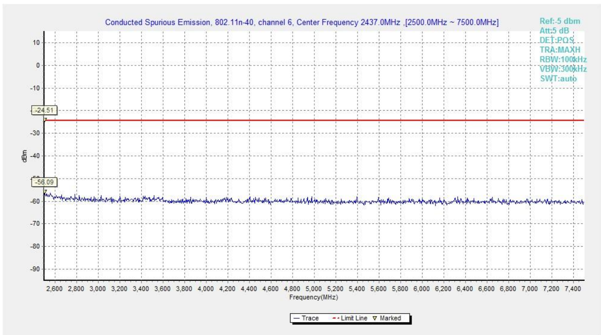
Fig.A.6.1.132 Transmitter Spurious Emission - Conducted (802.11n-HT40, Chain1, Ch6, 2.5 GHz-7.5 GHz)
