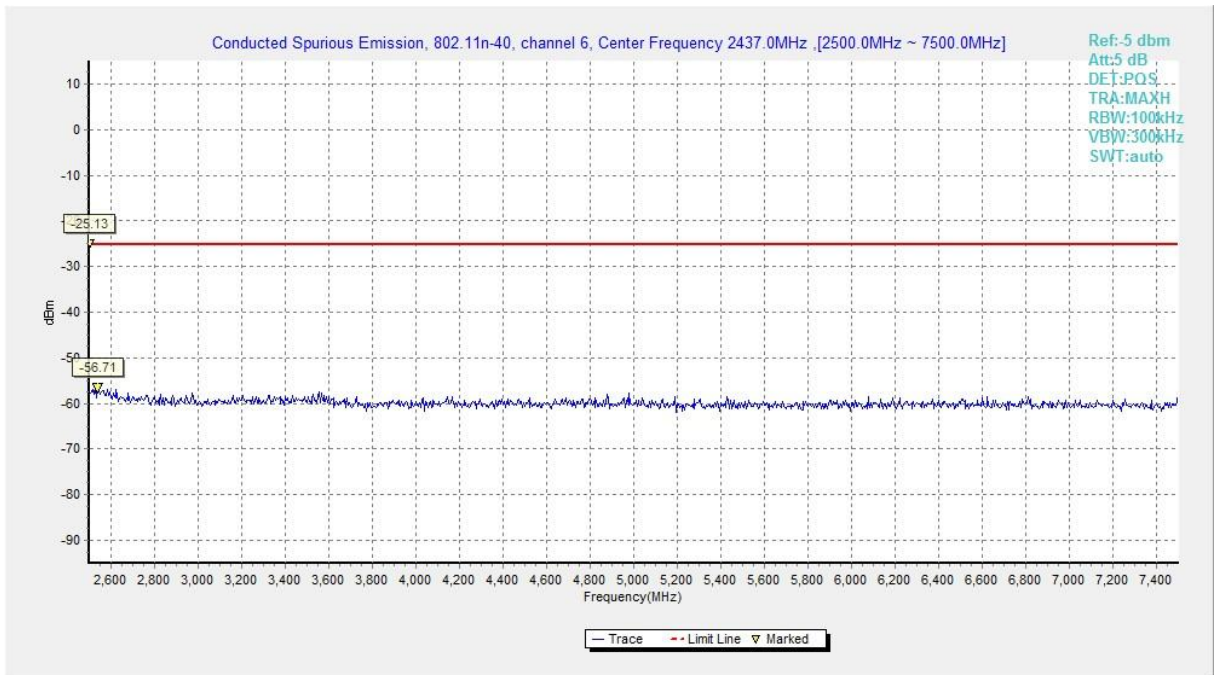
Fig.A.6.1.108 Transmitter Spurious Emission - Conducted (802.11n-HT40, Chain0, Ch6, 2.5 GHz-7.5 GHz)
