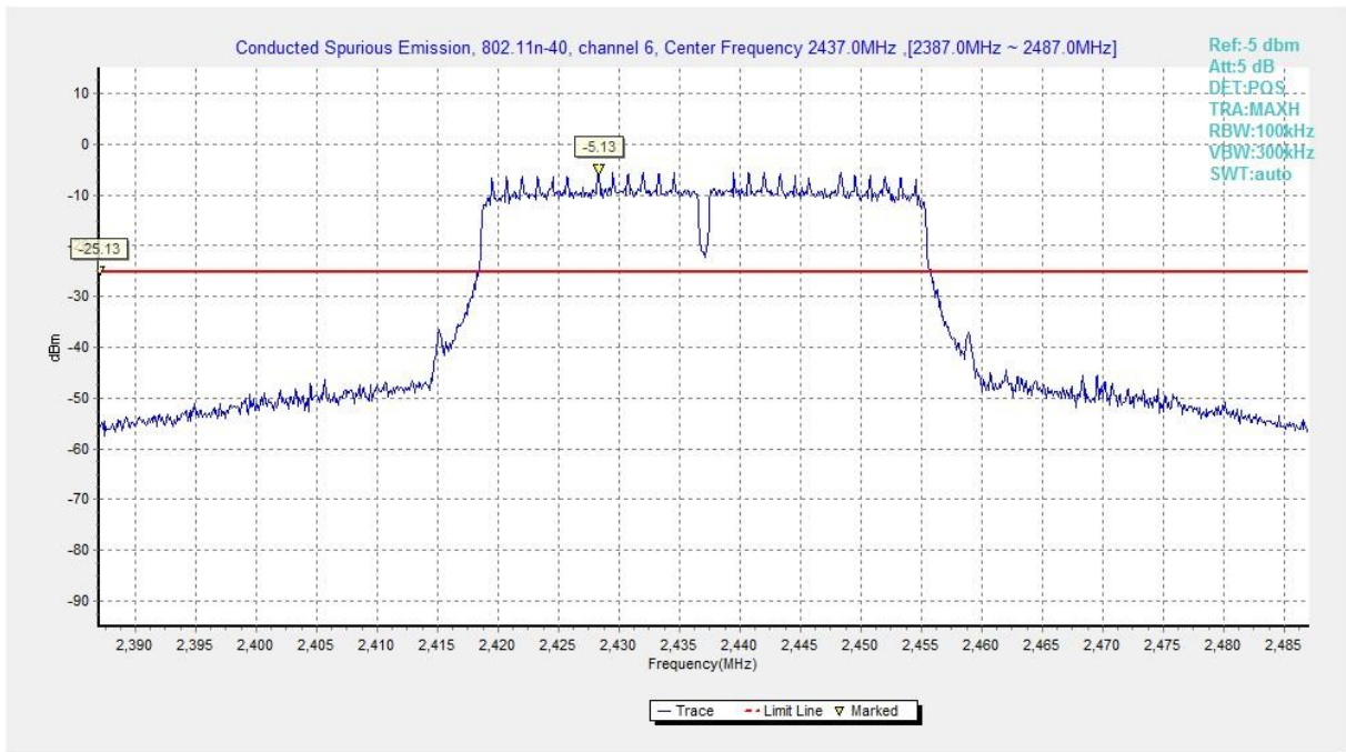
Fig.A.6.1.105 Transmitter Spurious Emission - Conducted (802.11n-HT40, Chain0, Ch6, Center Frequency)
