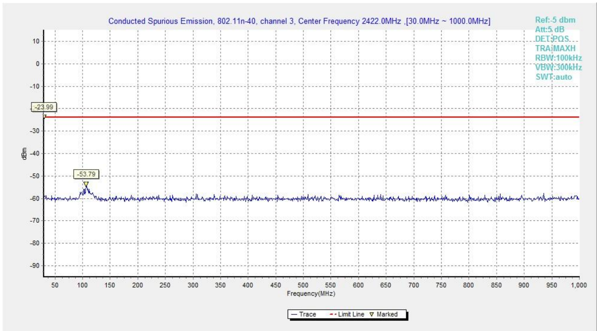
Fig.A.6.1.122 Transmitter Spurious Emission - Conducted (802.11n-HT40, Chain1, CH3, 30 MHz-1 GHz)
