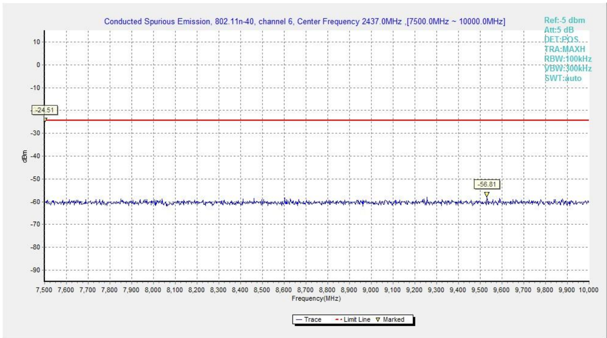
Fig.A.6.1.133 Transmitter Spurious Emission - Conducted (802.11n-HT40, Chain1, Ch6, 7.5 GHz-10 GHz)
