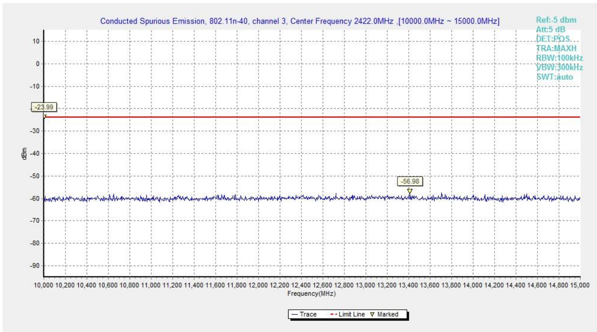
Fig.A.6.1.126 Transmitter Spurious Emission - Conducted (802.11n-HT40, Chain1, Ch3, 10 GHz-15 GHz)
