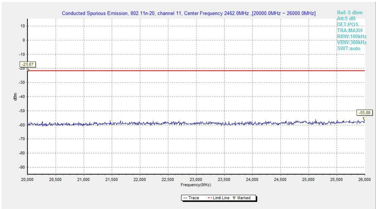
Fig.A.6.1.96 Transmitter Spurious Emission - Conducted (802.11n-HT20, Chain1, Ch11, 20 GHz-26 GHz)
