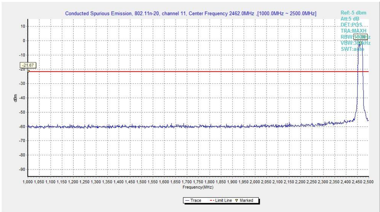
Fig.A.6.1.91 Transmitter Spurious Emission - Conducted (802.11n-HT20, Chain1, Ch11, 1 GHz-2.5 GHz)
