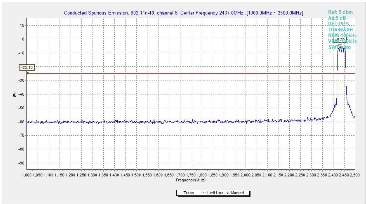
Fig.A.6.1.107 Transmitter Spurious Emission - Conducted (802.11n-HT40, Chain0, Ch6, 1 GHz-2.5 GHz)
