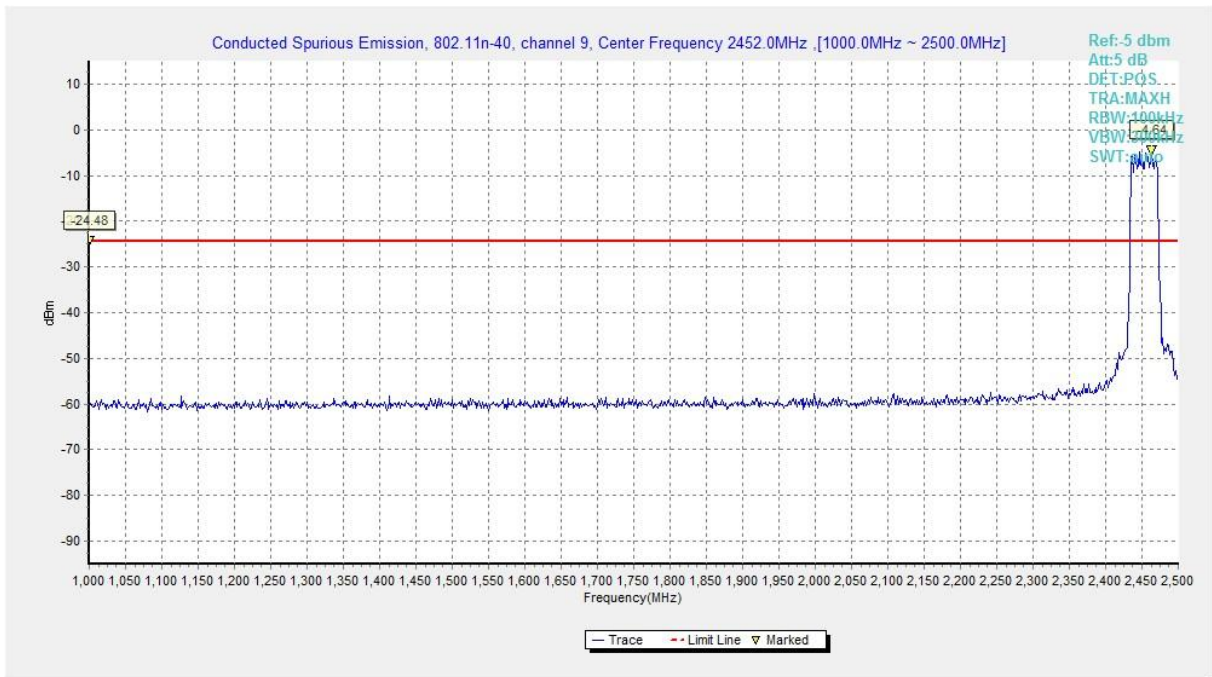
Fig.A.6.1.139 Transmitter Spurious Emission - Conducted (802.11n-HT40, Chain1, Ch9, 1 GHz-2.5 GHz)
