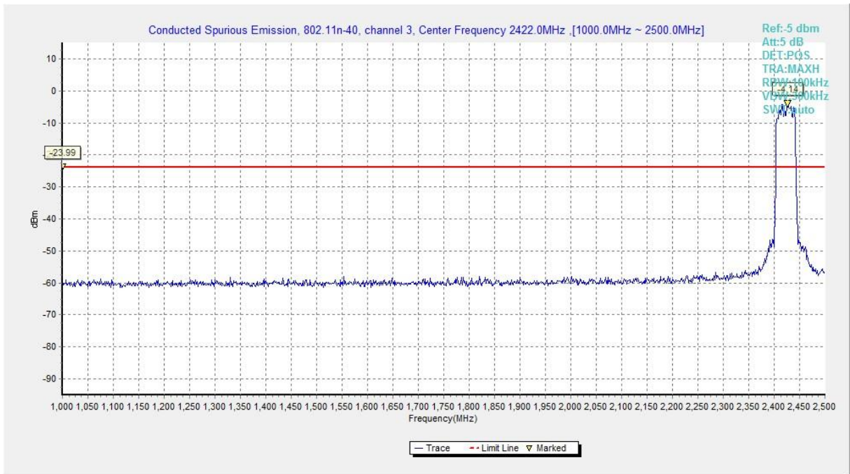
Fig.A.6.1.123 Transmitter Spurious Emission - Conducted (802.11n-HT40, Chain1, Ch3, 1 GHz-2.5 GHz)
