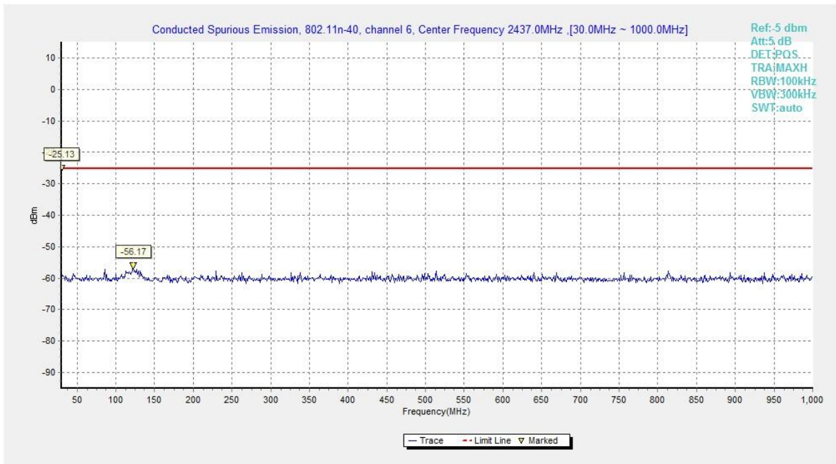
Fig.A.6.1.106 Transmitter Spurious Emission - Conducted (802.11n-HT40, Chain0, Ch6, 30 MHz-1 GHz)
