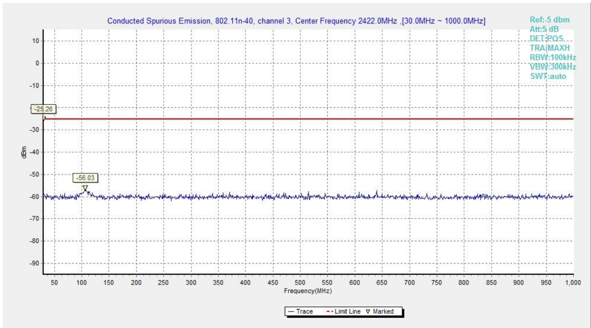
Fig.A.6.1.98 Transmitter Spurious Emission - Conducted (802.11n-HT40, Chain0, Ch3, 30 MHz-1 GHz)
