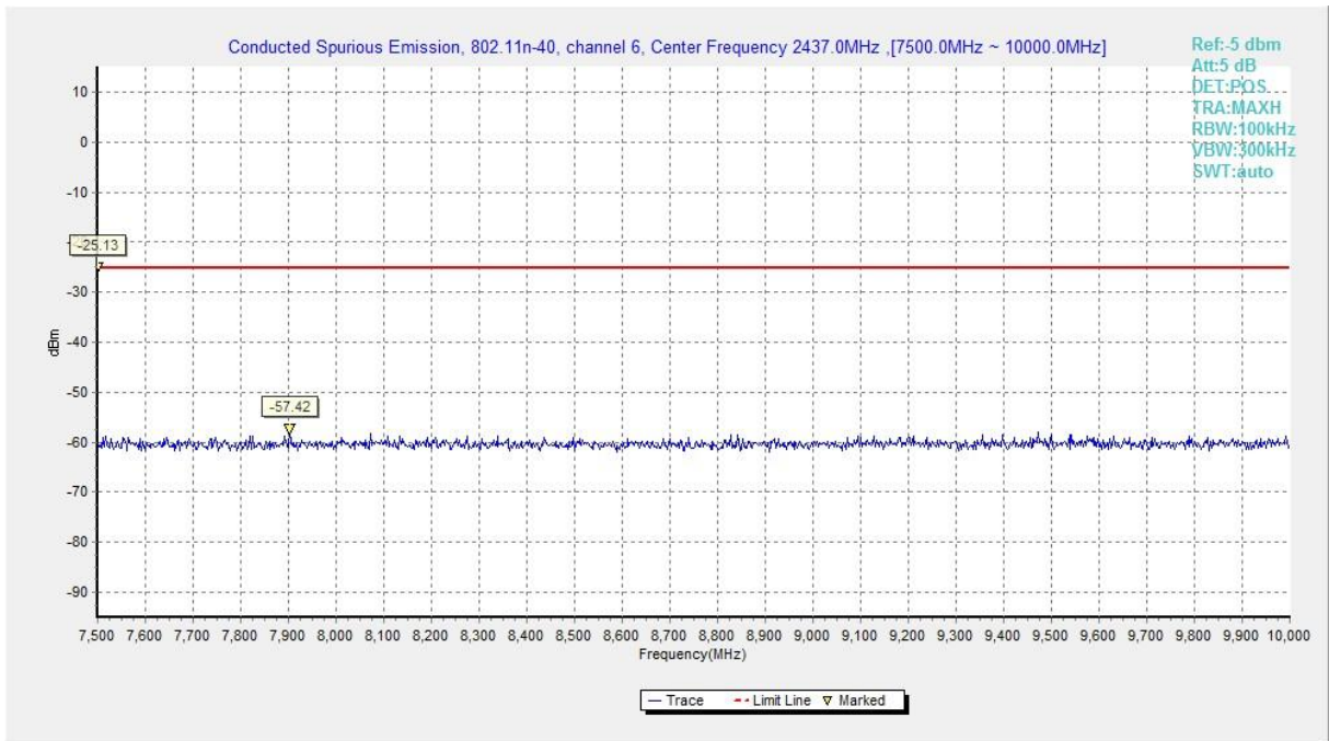
Fig.A.6.1.109 Transmitter Spurious Emission - Conducted (802.11n-HT40, Chain0, Ch6, 7.5 GHz-10 GHz)
