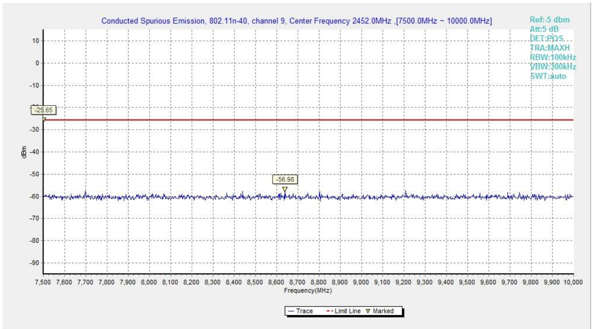
Fig.A.6.1.117 Transmitter Spurious Emission - Conducted (802.11n-HT40, Chain0, Ch9, 7.5 GHz-10 GHz)
