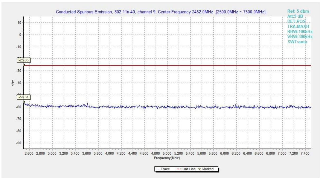
Fig.A.6.1.116 Transmitter Spurious Emission - Conducted (802.11n-HT40, Chain0, Ch9, 2.5 GHz-7.5 GHz)
