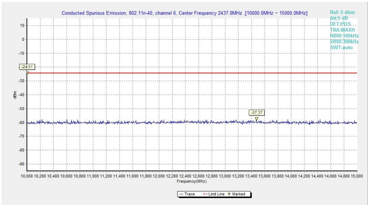
Fig.A.6.1.134 Transmitter Spurious Emission - Conducted (802.11n-HT40, Chain1, Ch6, 10 GHz-15 GHz)
