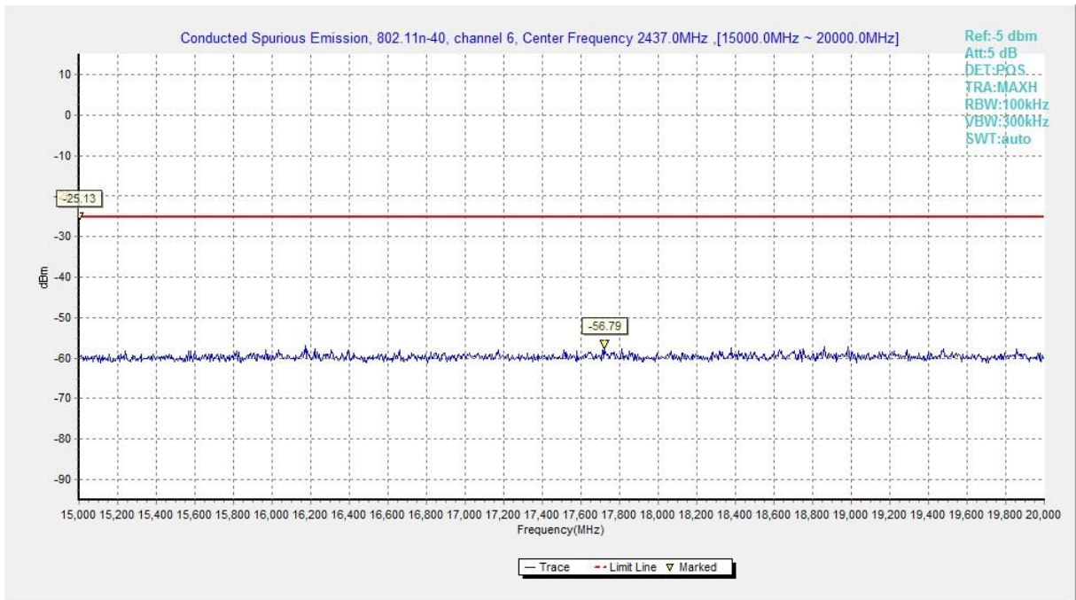
Fig.A.6.1.111 Transmitter Spurious Emission - Conducted (802.11n-HT40, Chain0, Ch6, 15 GHz-20 GHz)
