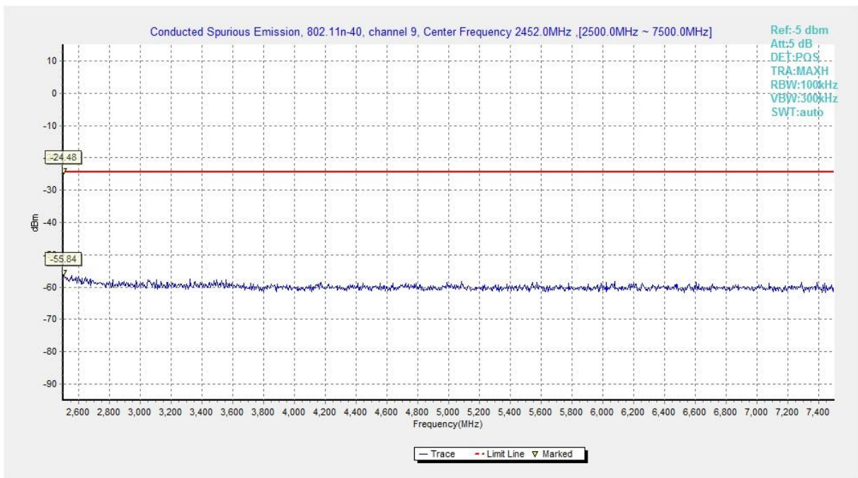
Fig.A.6.1.140 Transmitter Spurious Emission - Conducted (802.11n-HT40, Chain1, Ch9, 2.5 GHz-7.5 GHz)
