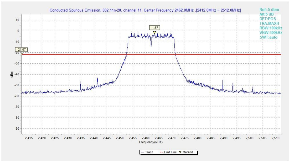
Fig.A.6.1.89 Transmitter Spurious Emission - Conducted (802.11n-HT20, Chain1, Ch11, Center Frequency)
