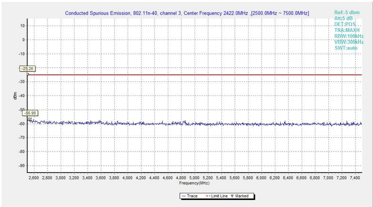
Fig.A.6.1.100 Transmitter Spurious Emission - Conducted (802.11n-HT40, Chain0, Ch3, 2.5 GHz-7.5 GHz)
