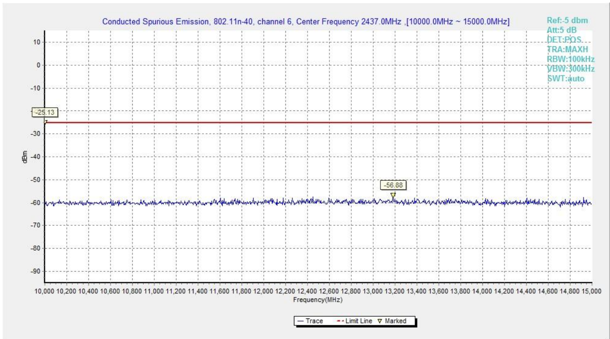
Fig.A.6.1.110 Transmitter Spurious Emission - Conducted (802.11n-HT40, Chain0, Ch6, 10 GHz-15 GHz)
