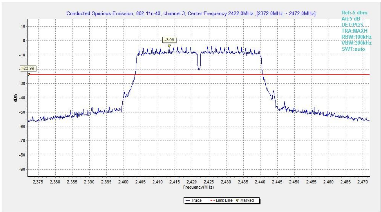
Fig.A.6.1.121 Transmitter Spurious Emission - Conducted (802.11n-HT40, Chain1, Ch3, Center Frequency)
