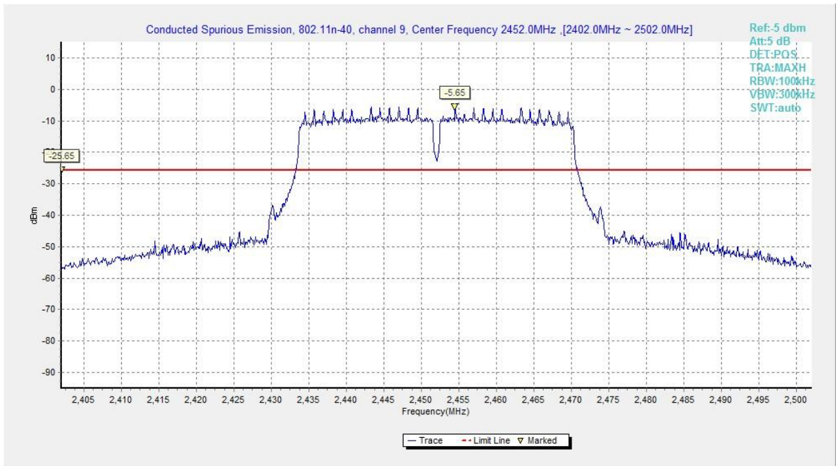
Fig.A.6.1.113 Transmitter Spurious Emission - Conducted (802.11n-HT40, Chain0, Ch9, Center Frequency)
