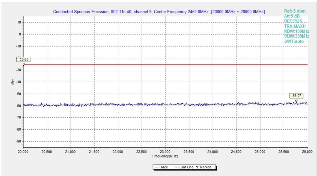
Fig.A.6.1.120 Transmitter Spurious Emission - Conducted (802.11n-HT40, Chain0, Ch9, 20 GHz-26 GHz)
