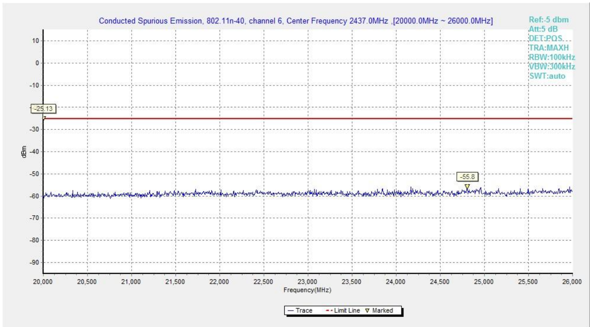
Fig.A.6.1.112 Transmitter Spurious Emission - Conducted (802.11n-HT40, Chain0, Ch6, 20 GHz-26 GHz)
