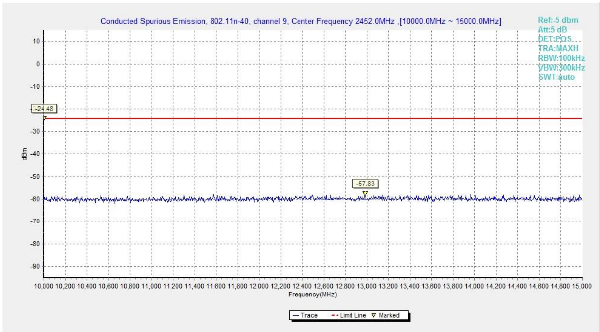
Fig.A.6.1.142 Transmitter Spurious Emission - Conducted (802.11n-HT40, Chain1, Ch9, 10 GHz-15 GHz)
