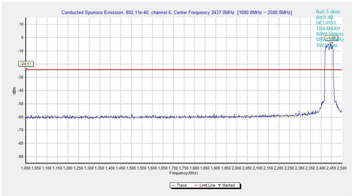
Fig.A.6.1.131 Transmitter Spurious Emission - Conducted (802.11n-HT40, Chain1, Ch6, 1 GHz-2.5 GHz)
