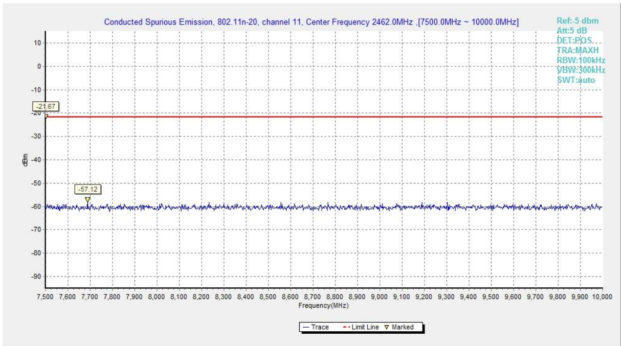
Fig.A.6.1.93 Transmitter Spurious Emission - Conducted (802.11n-HT20, Chain1, Ch11, 7.5 GHz-10 GHz)
