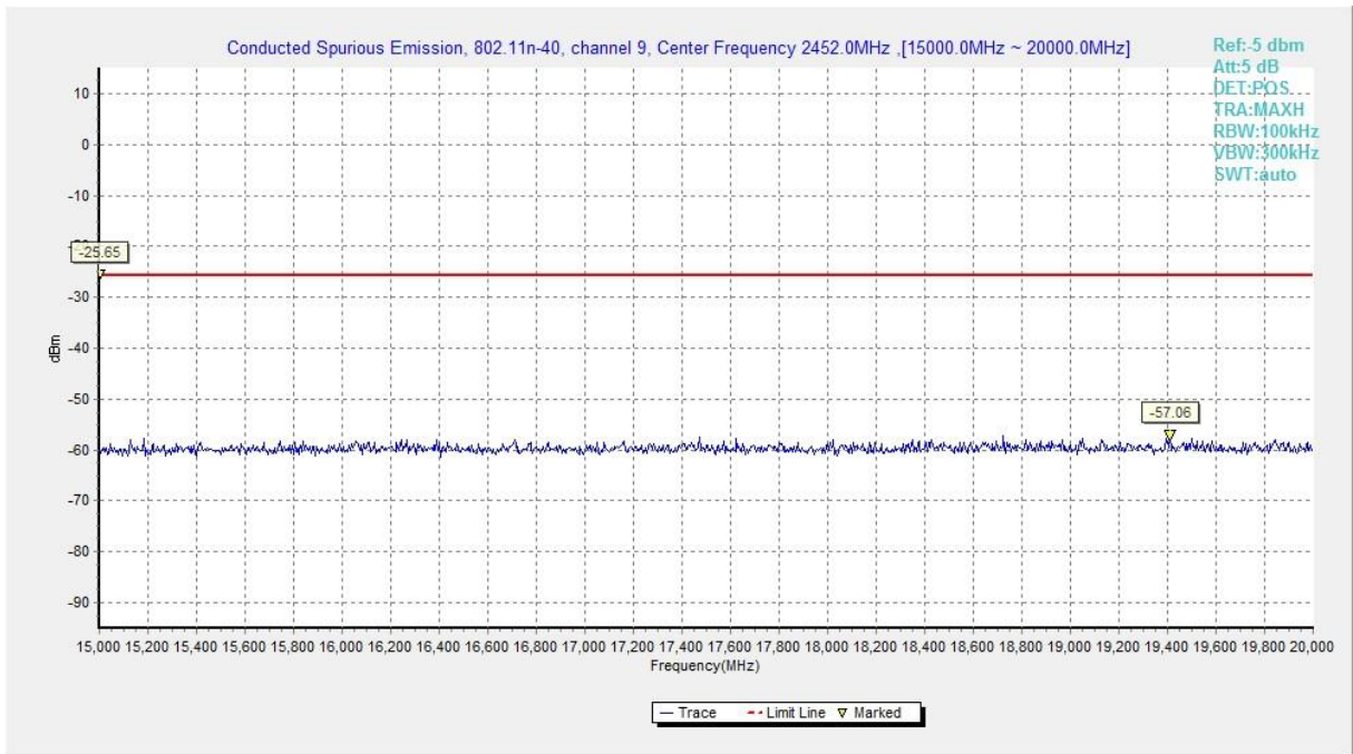
Fig.A.6.1.119 Transmitter Spurious Emission - Conducted (802.11n-HT40, Chain0, Ch9, 15 GHz-20 GHz)
