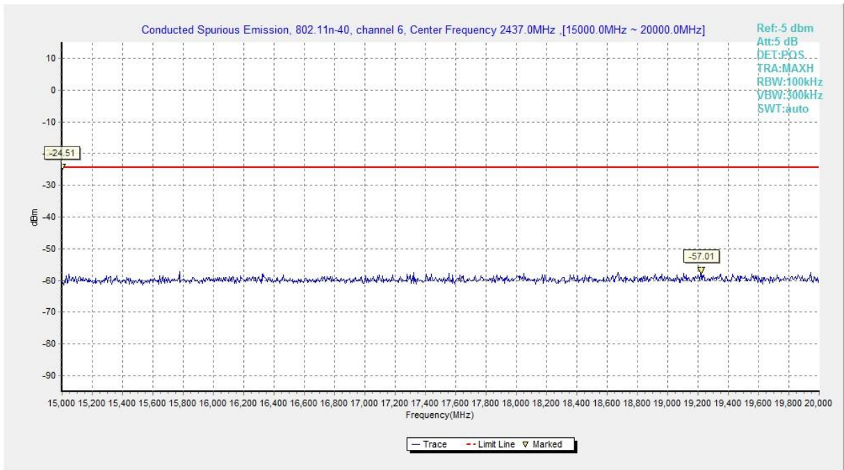
Fig.A.6.1.135 Transmitter Spurious Emission - Conducted (802.11n-HT40, Chain1, Ch6, 15 GHz-20 GHz)
