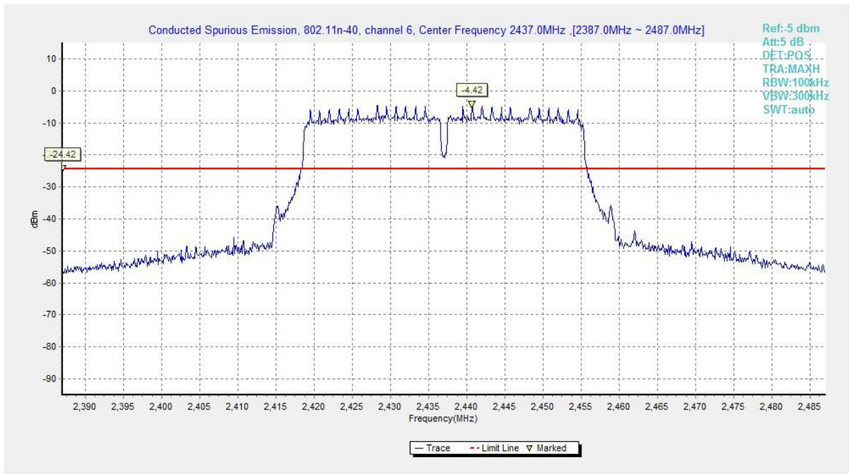
Fig.A.6.1.129 Transmitter Spurious Emission - Conducted (802.11n-HT40, Chain1, Ch6, Center Frequency)
