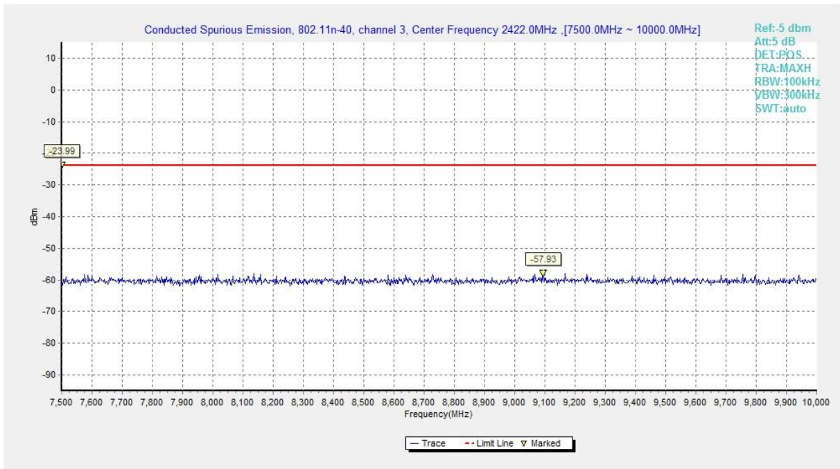
Fig.A.6.1.125 Transmitter Spurious Emission - Conducted (802.11n-HT40, Chain1, Ch3, 7.5 GHz-10 GHz)
