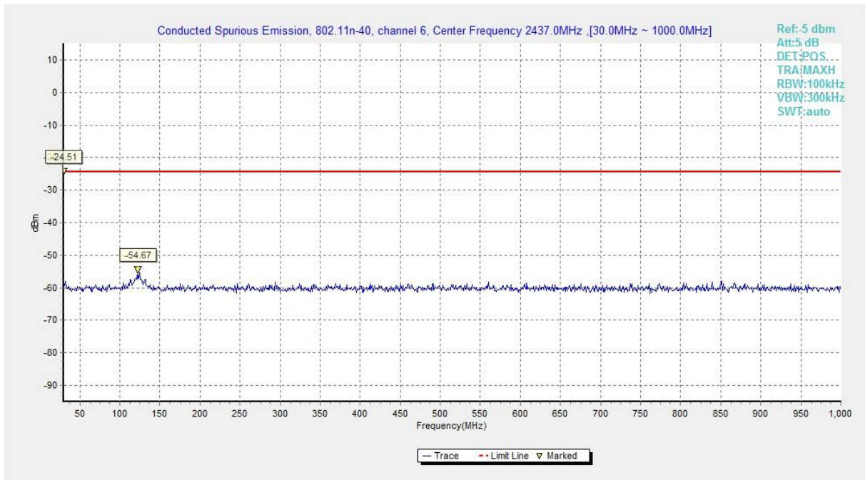
Fig.A.6.1.130 Transmitter Spurious Emission - Conducted (802.11n-HT40, Chain1, Ch6, 30 MHz-1 GHz)
