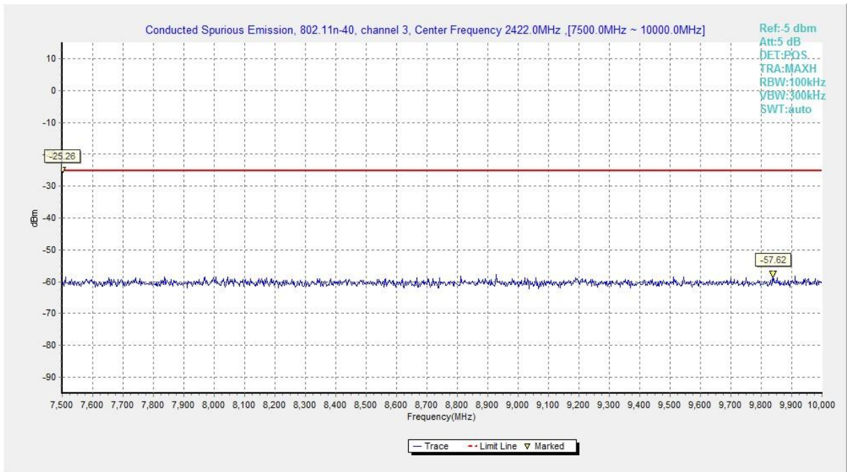
Fig.A.6.1.101 Transmitter Spurious Emission - Conducted (802.11n-HT40, Chain0, Ch3, 7.5 GHz-10 GHz)
