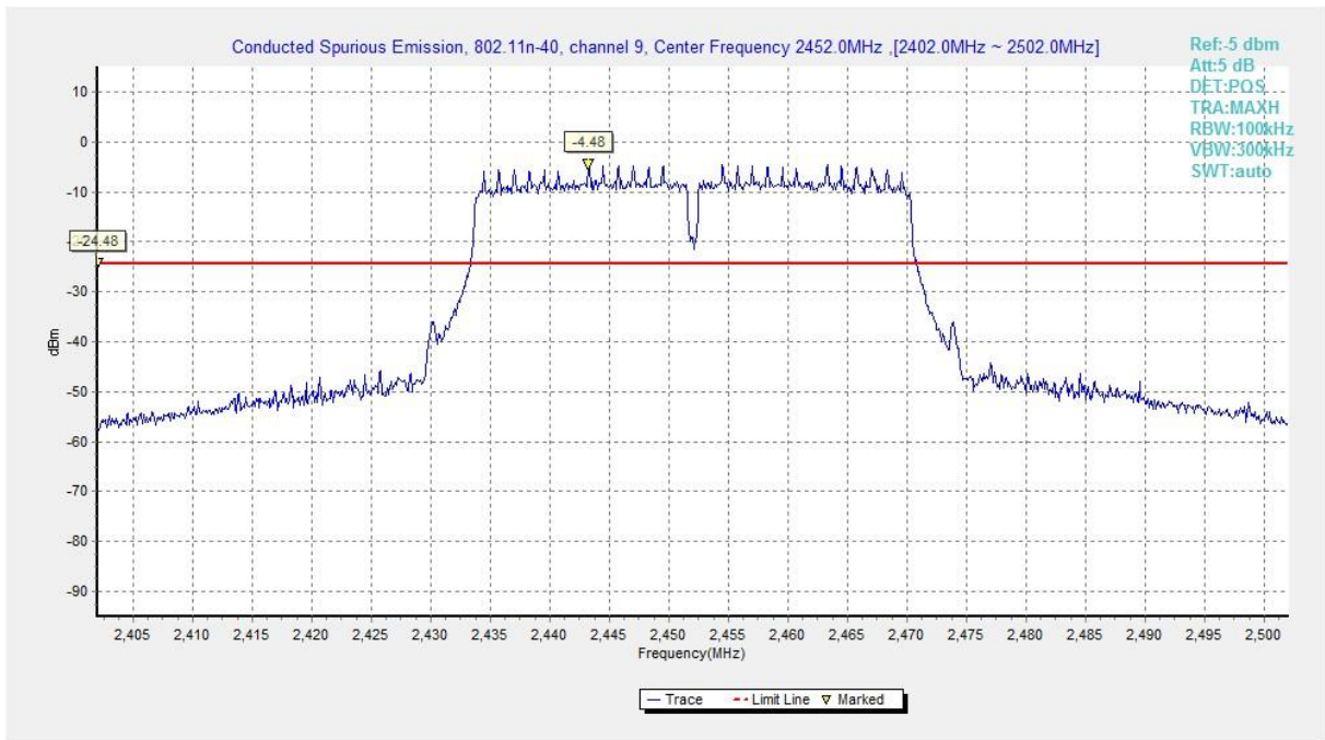
Fig.A.6.1.137 Transmitter Spurious Emission - Conducted (802.11n-HT40, Chain1, Ch9, Center Frequency)
