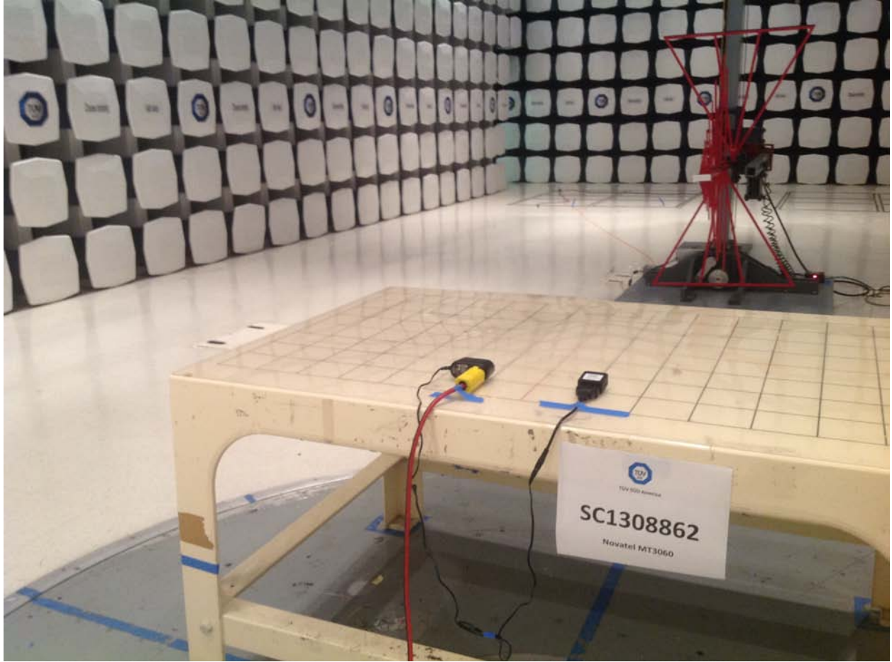
Radiated Emissions <1GHz Test Setup
