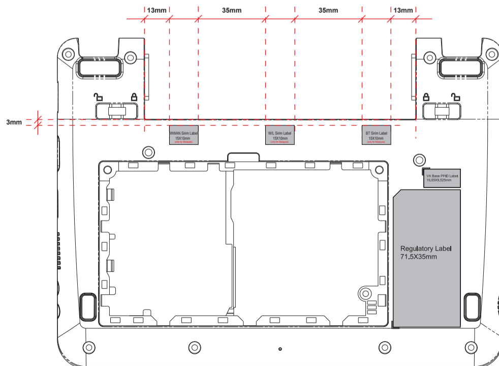
RAM door outside view
