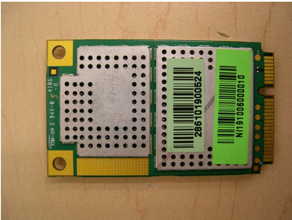
E725 - Bottom side with shields
