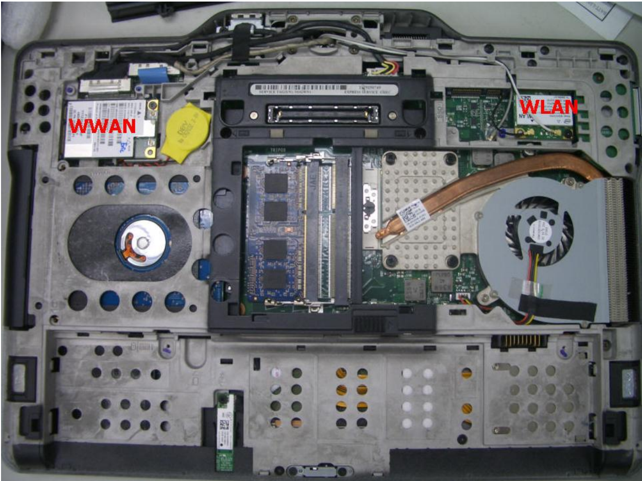
Placement of WWAN and WLAN modules. This is the view from the bottom of the laptop.
