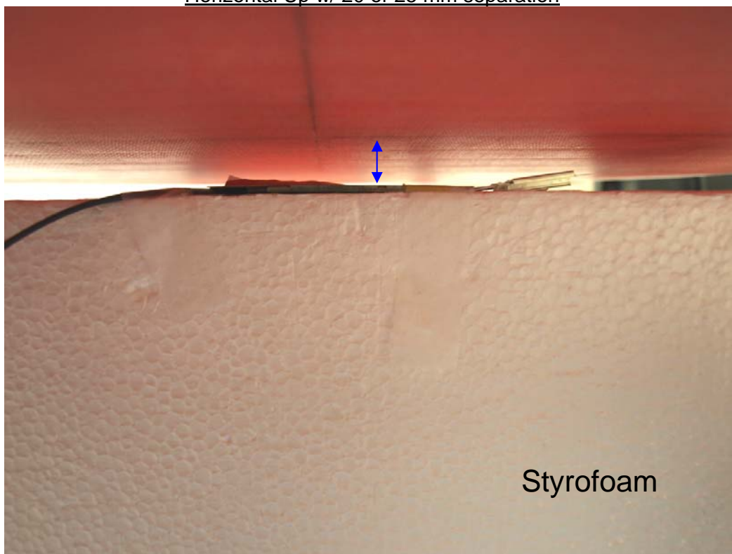
Horizontal Up w/ 20 or 25 mm separation
