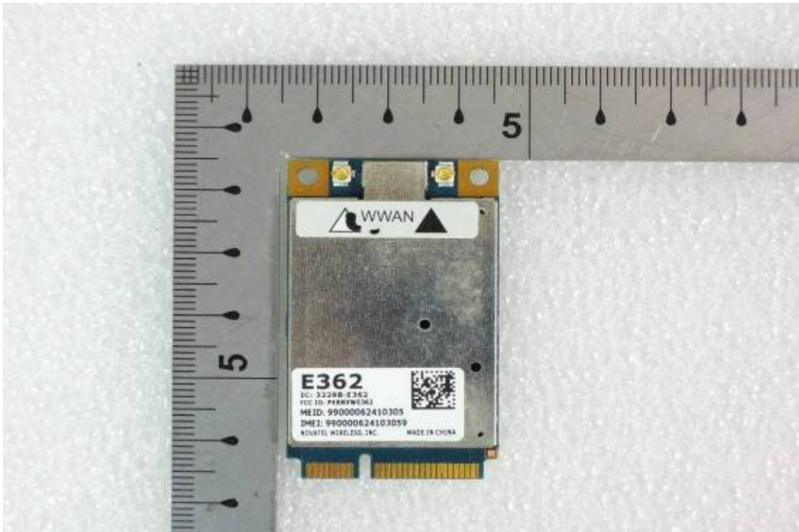
Front view of WWAN Module
