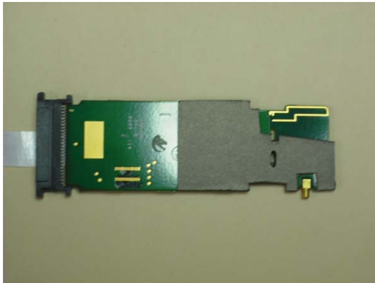
Back of PCB With Absorber Installed
