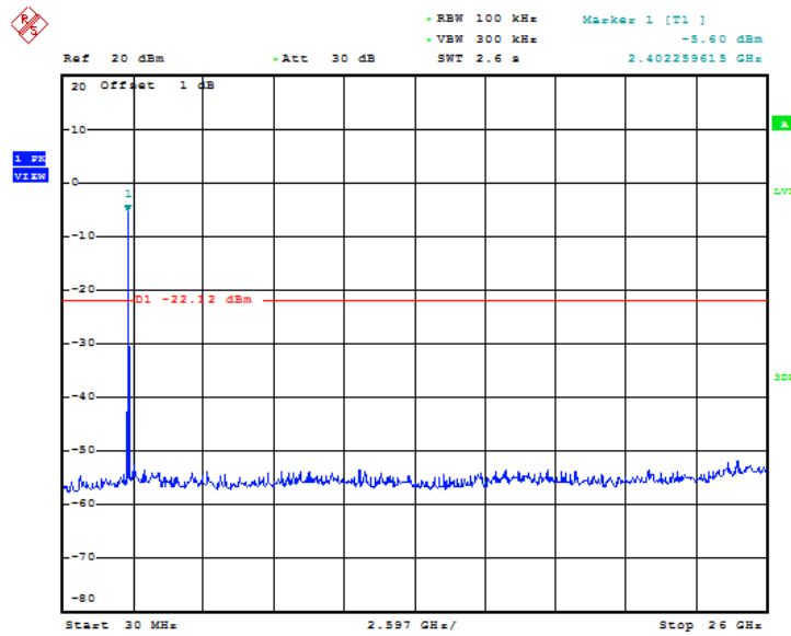
Fig 34. Conducted Spurious Emission (802.11b, Ch1)
