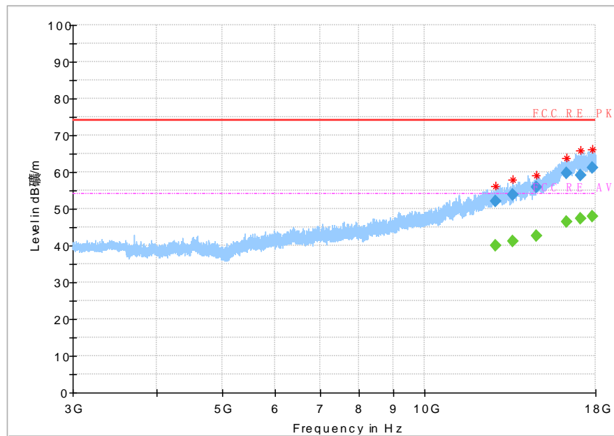
Fig 69. Radiated Spurious Emission (802.11 n-20MHz,Ch11, 3GHz~18GHz)
