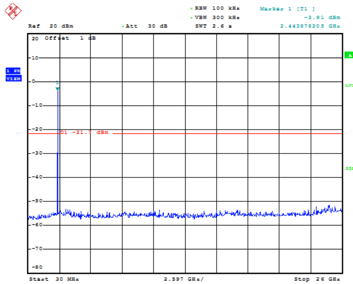
Fig 38. Conducted Spurious Emission (802.11b, Ch11)
