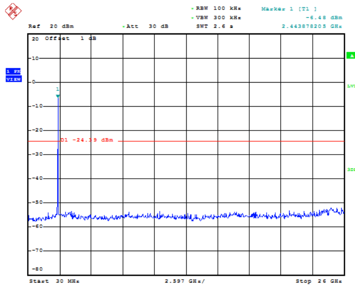
Fig 50. Conducted Spurious Emission (802.11n-20MHz, Ch11)
