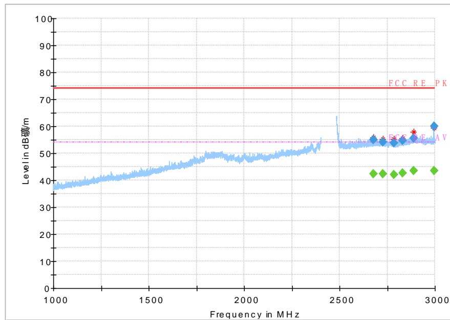
Fig 63. Radiated Spurious Emission (802.11g,Ch11,1GHz~3GHz)
