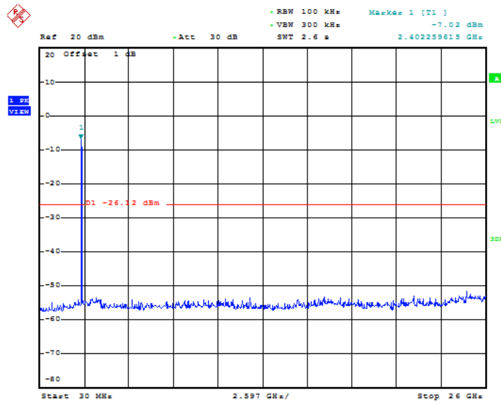
Fig 42. Conducted Spurious Emission (802.11g, Ch6)
