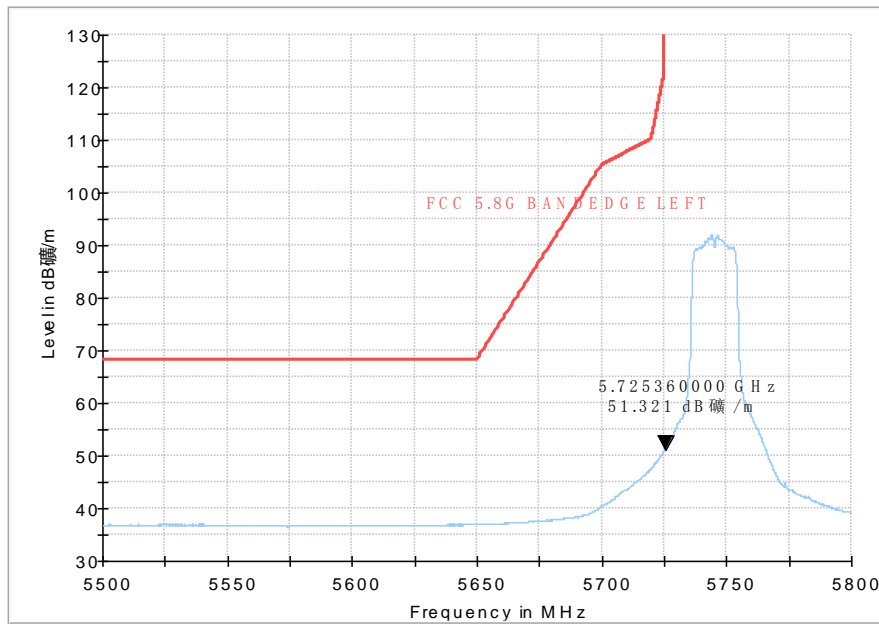
Average Fig. 54 Band Edges (802.11n-HT20, 5745MHz)
