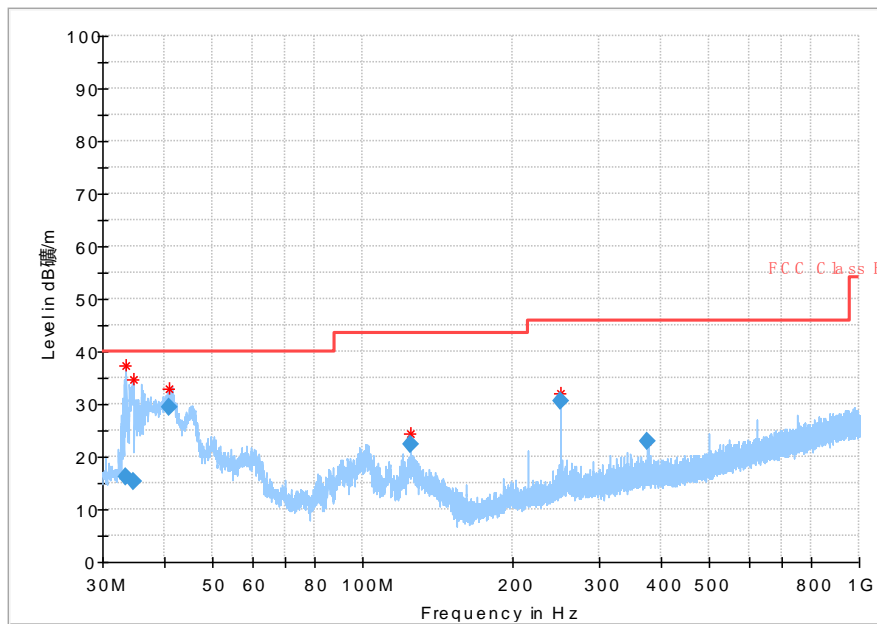
Fig. 42 Radiated Spurious Emission (802.11n-HT20, Ch165, 30 MHz-1 GHz)
