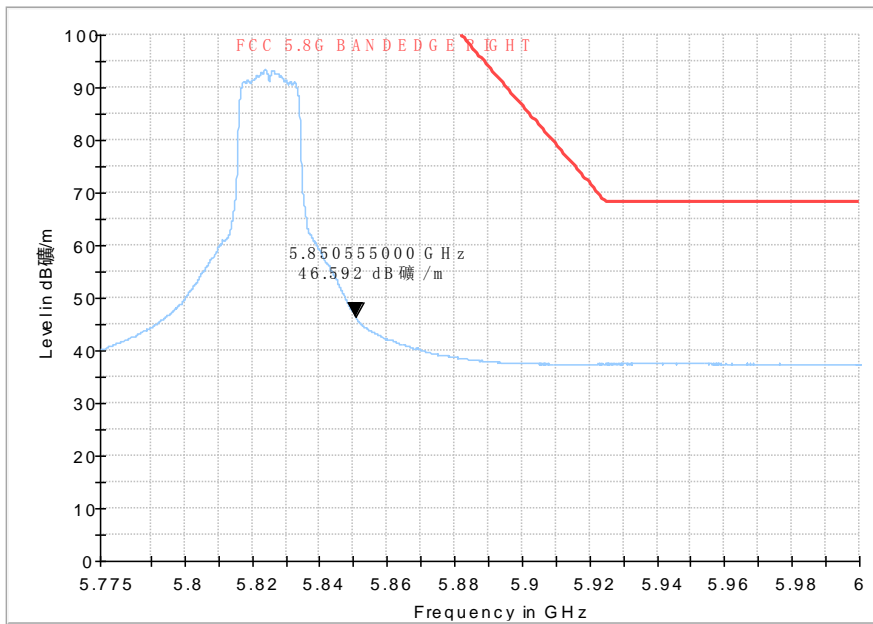
Average Fig. 55 Band Edges (802.11n-HT20, 5825MHz)
