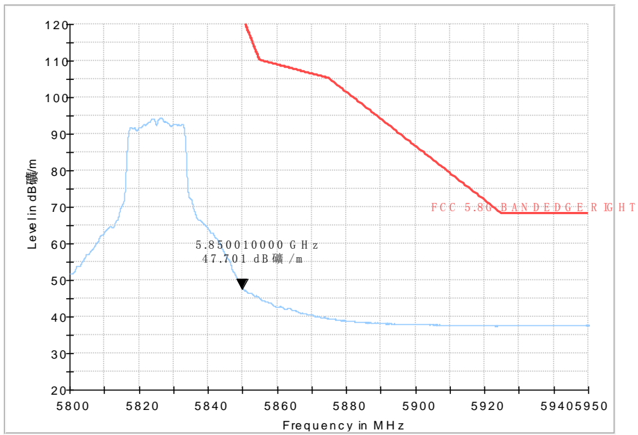
Average Fig. 53 Band Edges (802.11a, 5825MHz)
