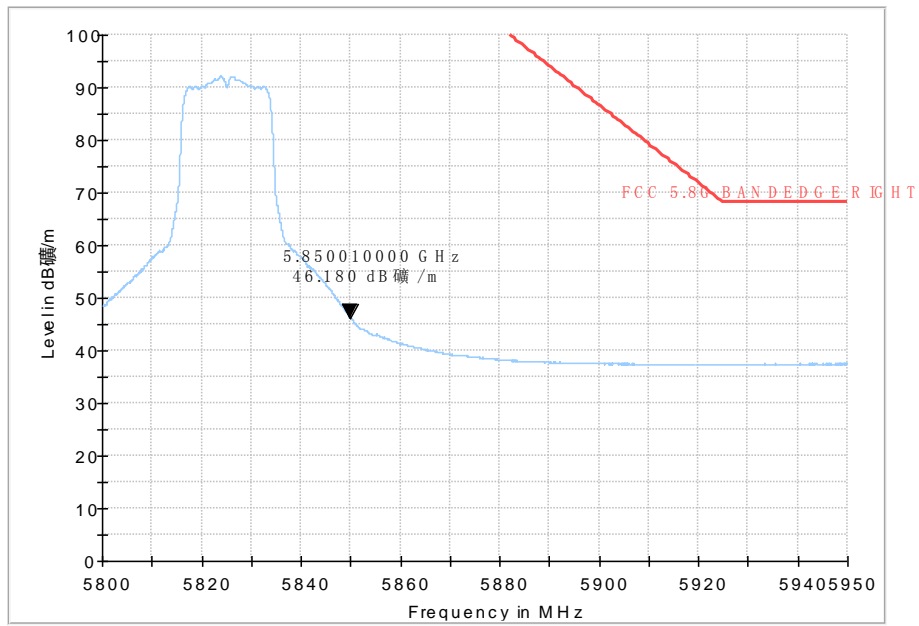
Fig. 57 Band Edges (802.11ac-HT20, 5825MHz)
