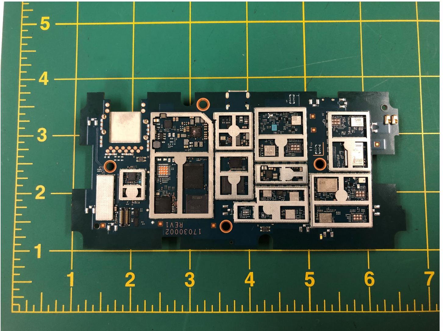
Figure 3 - PCB TOP Unshielded 1
