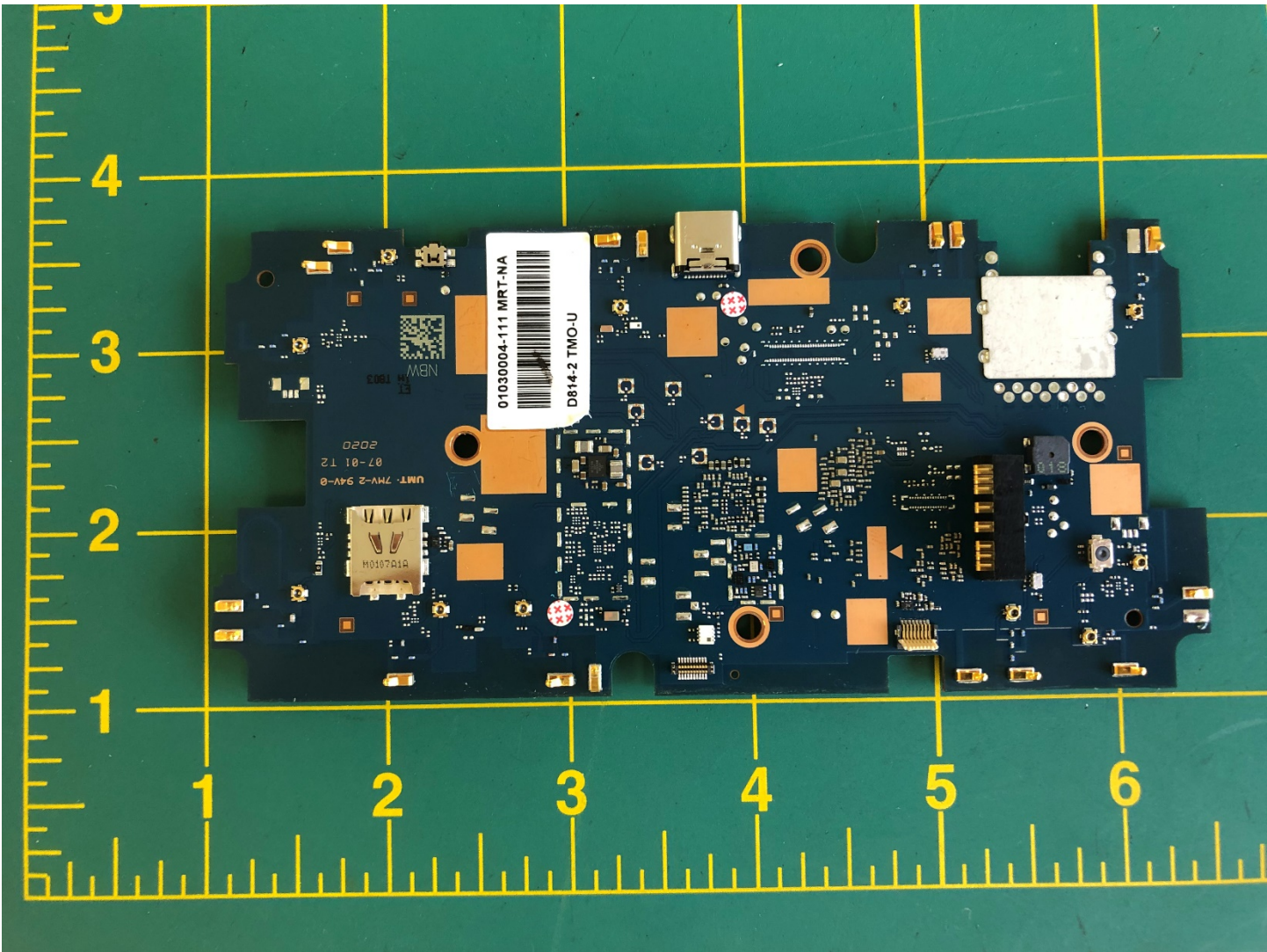
Figure 5 - PCB Bottom Unshielded
