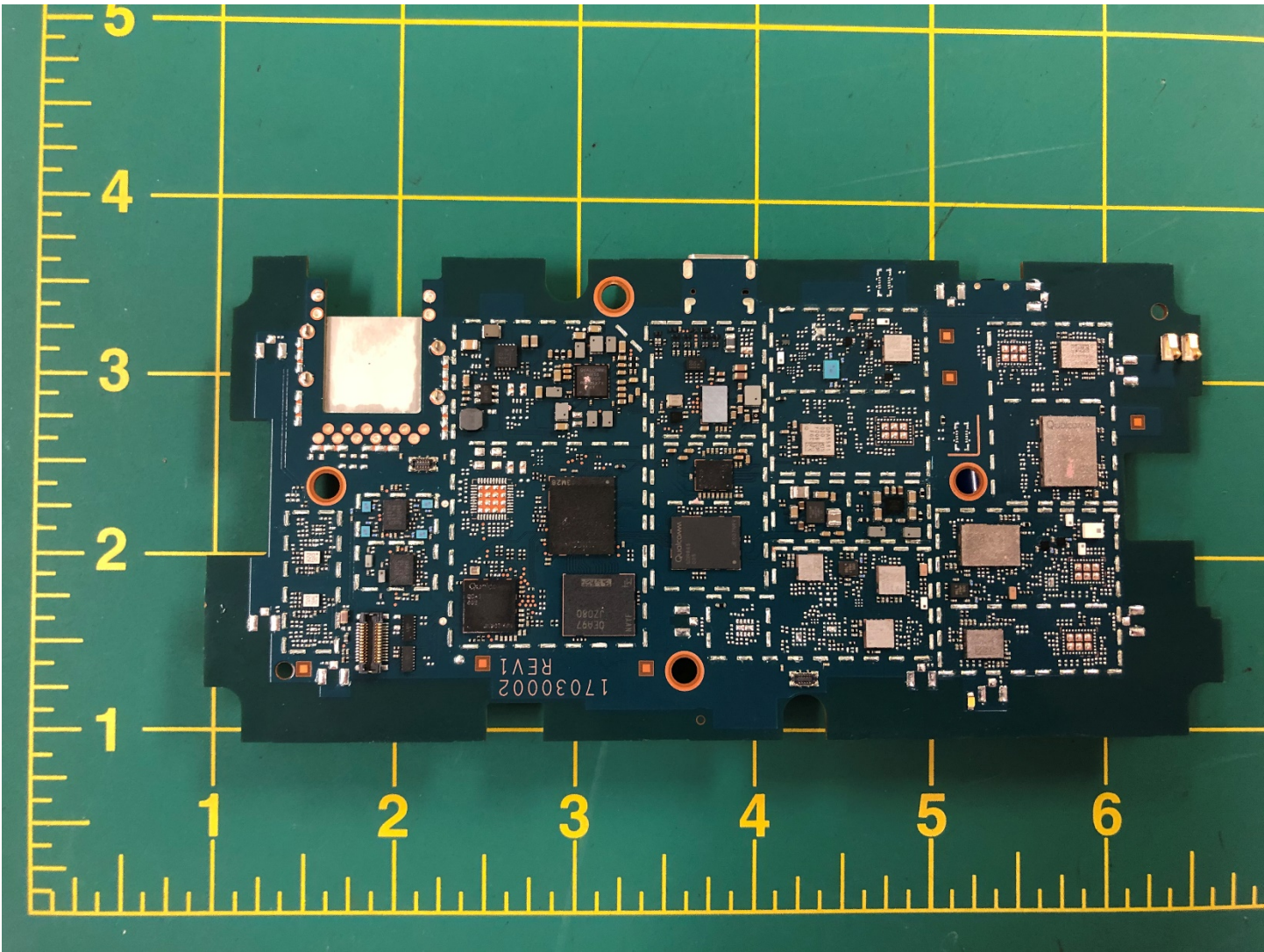
Figure 4 - PCB TOP Unshielded 2
