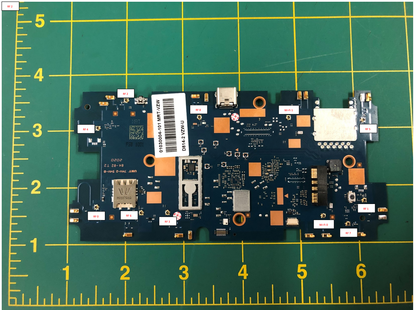
Figure 2 - PCB Bottom
