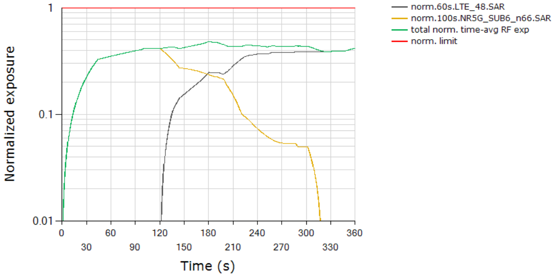
Total Normalized Time-averaged RF Exposure Tech: LTE, Band 48 / Tech: NR5G SUB6, Band n66
