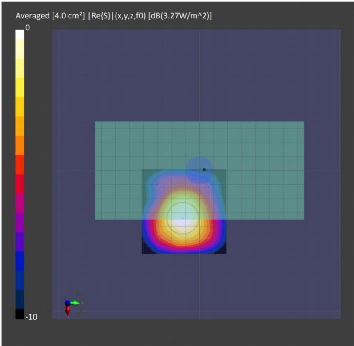
Figure 8-2: 4cm 2 -averaged power density distribution measured at input.power.limit of 11.555 dBm on the Top Side surface for n260 beam 0
