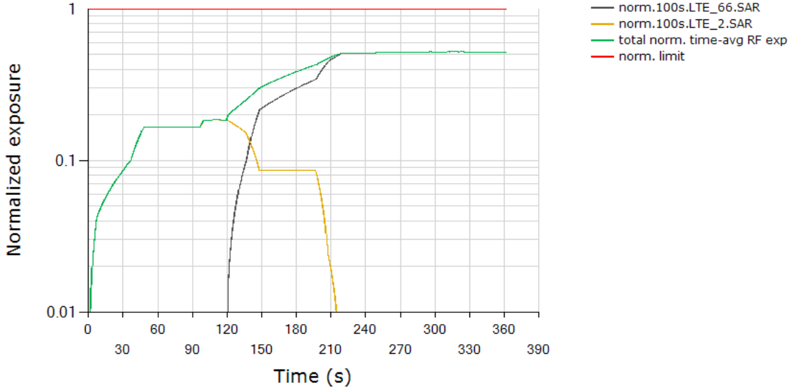
Total Normalized Time-averaged RF Exposure Tech: LTE, Band 66 / Tech: LTE, Band 2
