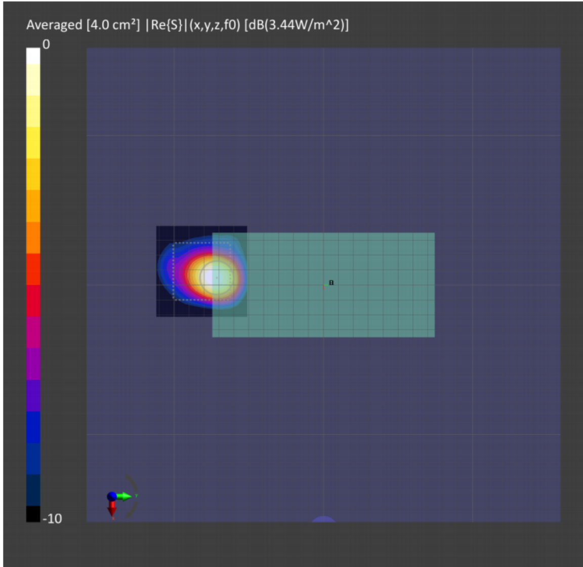
Figure 7-2: 4cm2-averaged power density distribution measured at input.power.limit of 7.6 dBm on the Top surface for n258 beam 20
