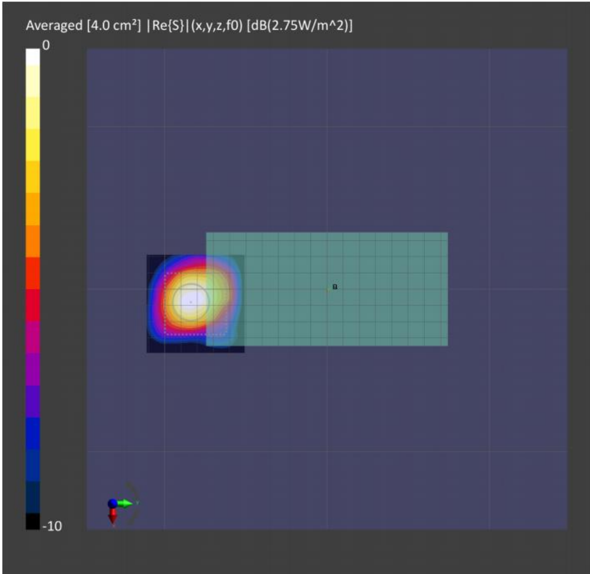
Figure 7-3: 4cm2-averaged power density distribution measured at input.power.limit of 7.68 dBm on the Top surface for n260 beam 28
