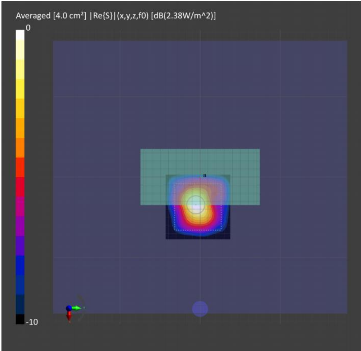
Figure 7-4: 4cm2-averaged power density distribution measured at input.power.limit of 13.34 dBm on the Top for n261 beam 0
