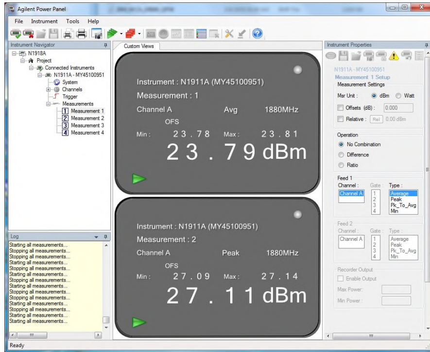
LTE Band 2_5M Bandwidth Middle Chanel QPSK 1 RB 12 offset
