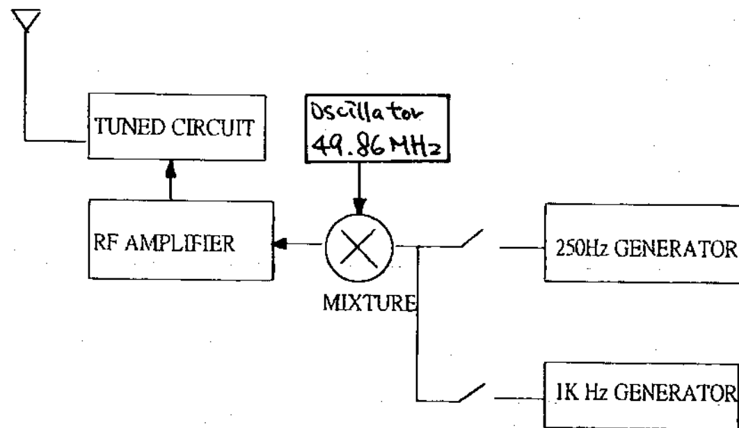
SERVING SANTA TRANSMITTER BLOCK DIAGRAM
