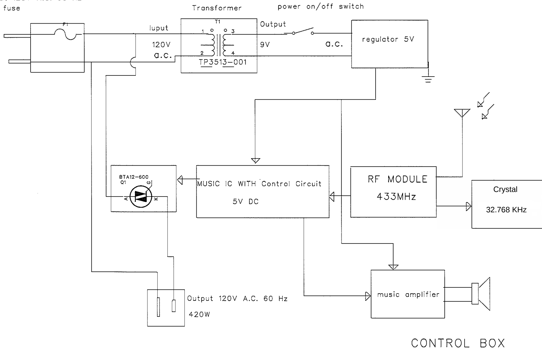
BLOCK DIAGRAM :Indoor Remote control Lns receiver
