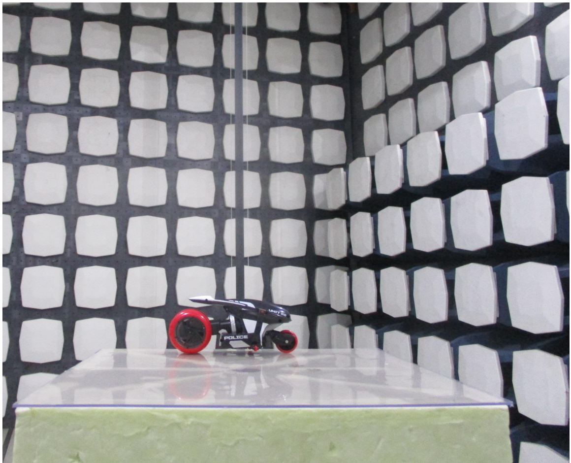
Above 1GHz (The EUT placed at the center of the turntable)
