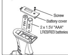
Diagram 1 BATTERY INSTALLATION
