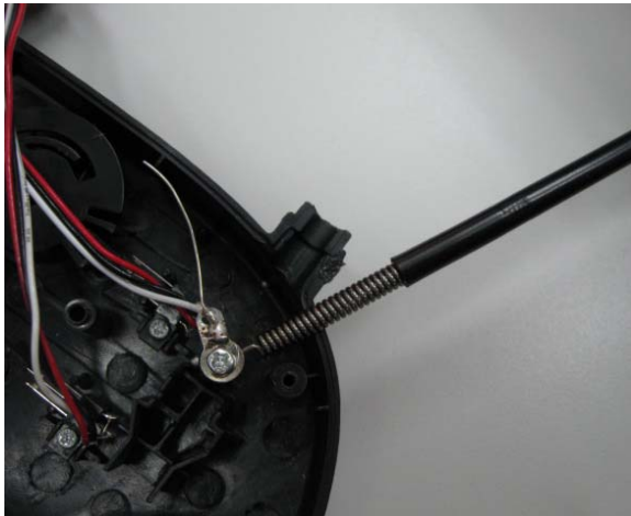
Antenna Photo
