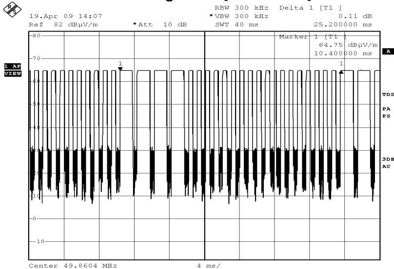
Figure A [Pulse Train]
