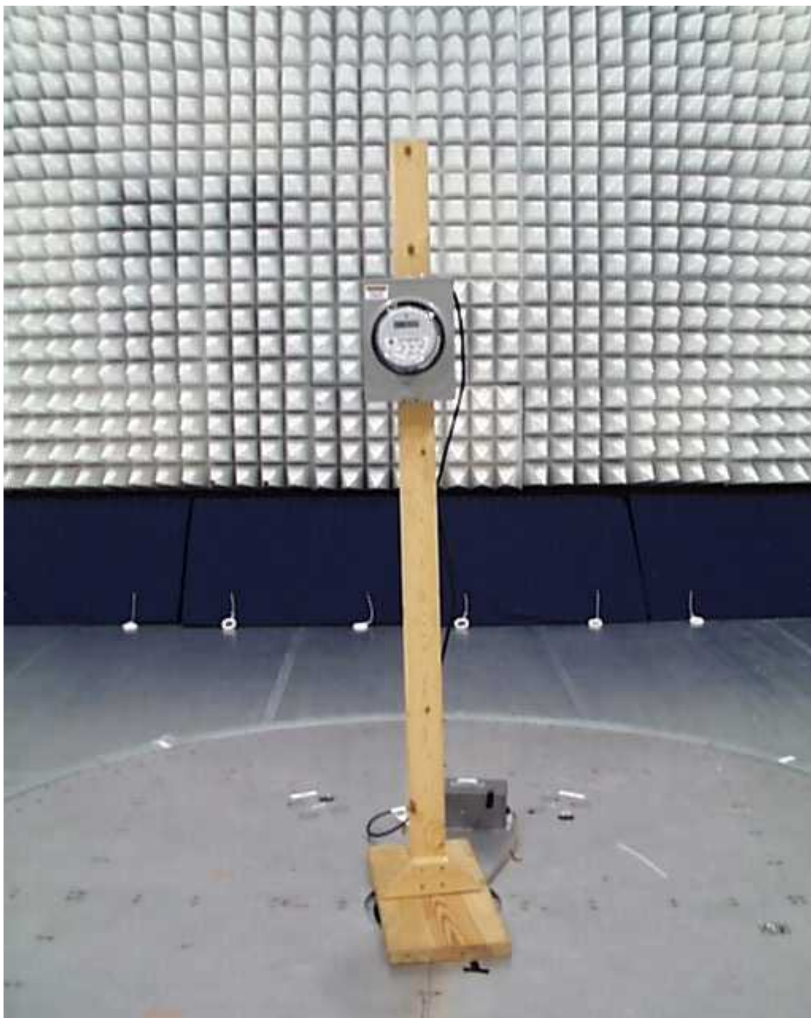
Radiated Emissions (Front View)
