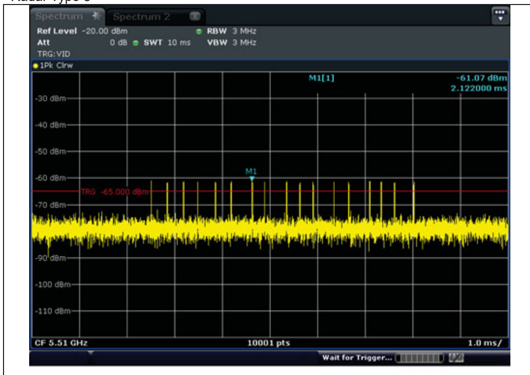
Radar Type 3
