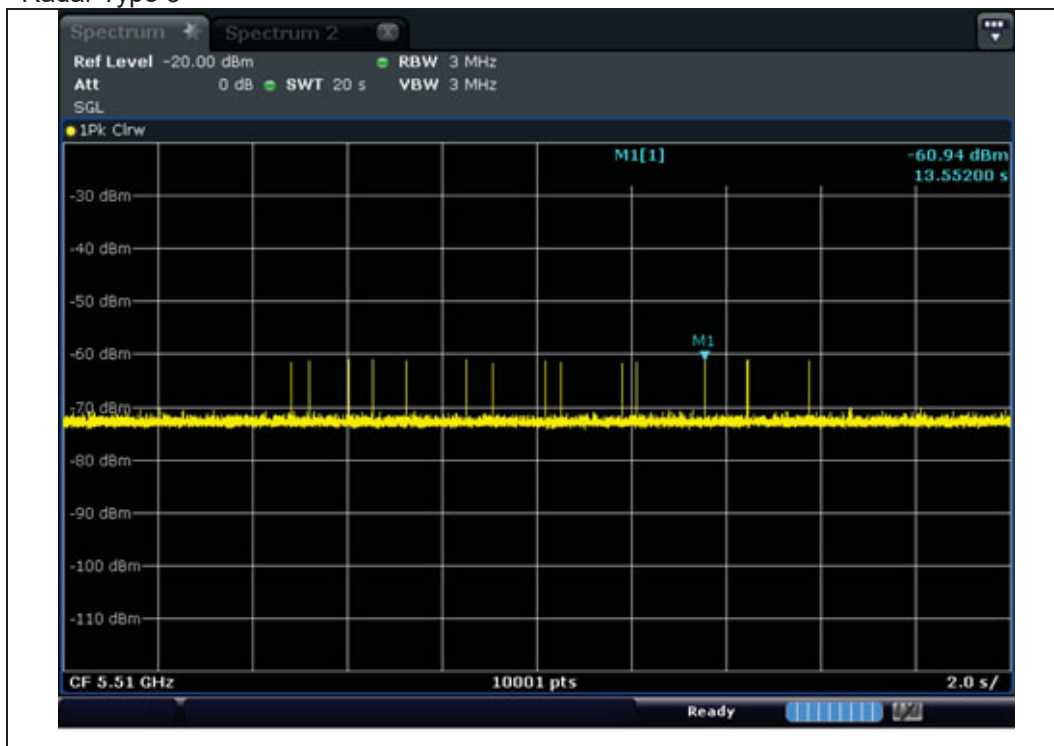
Radar Type 5
