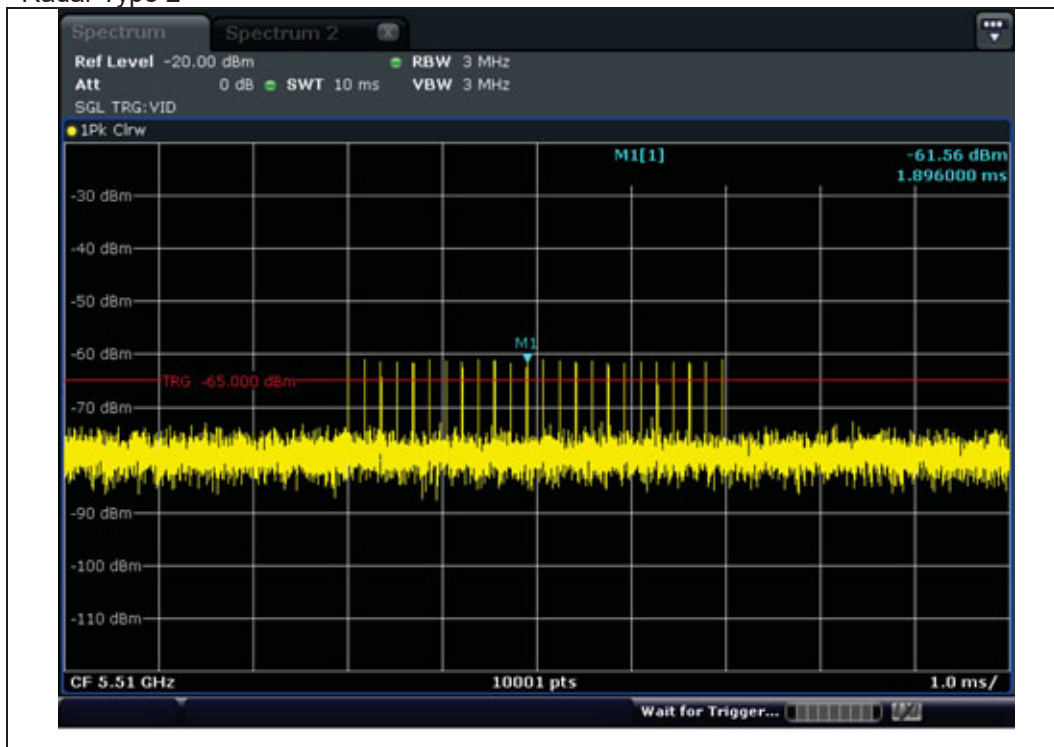
Radar Type 2
