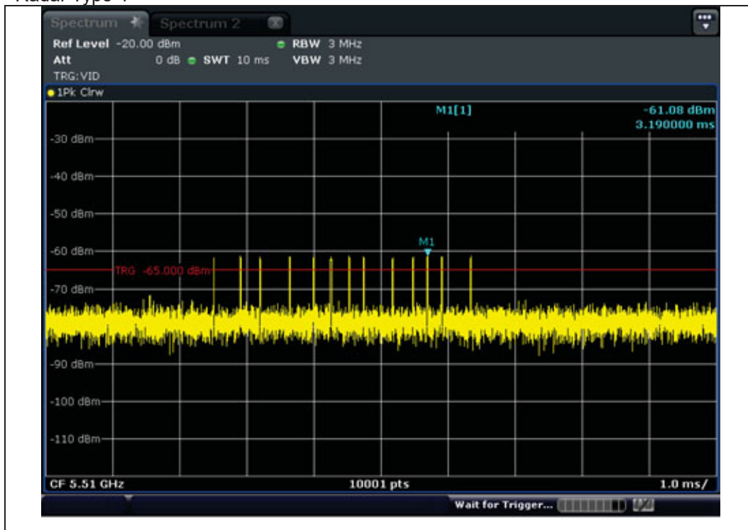
Radar Type 4
