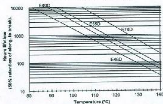
Graph 2.77: Heat stability for Arnitel E-range.
