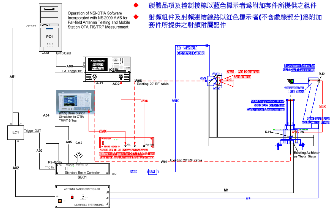
Configuration of NSI-800F 3D-chamber
