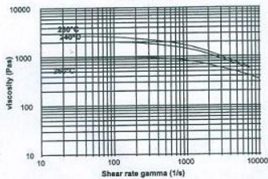
Shear rate dependent of the melt viscosity of Amitel EL630. Effect of melt temperature.
