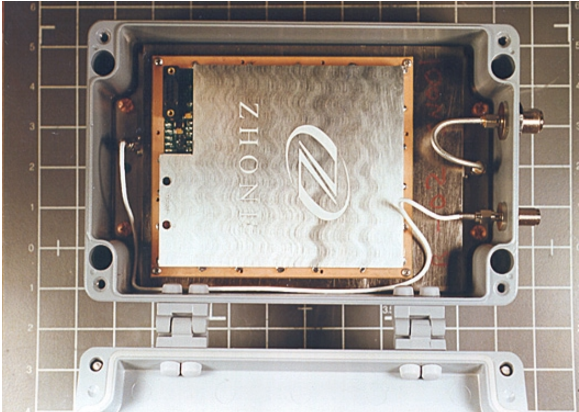
ODU B – Inside Front
