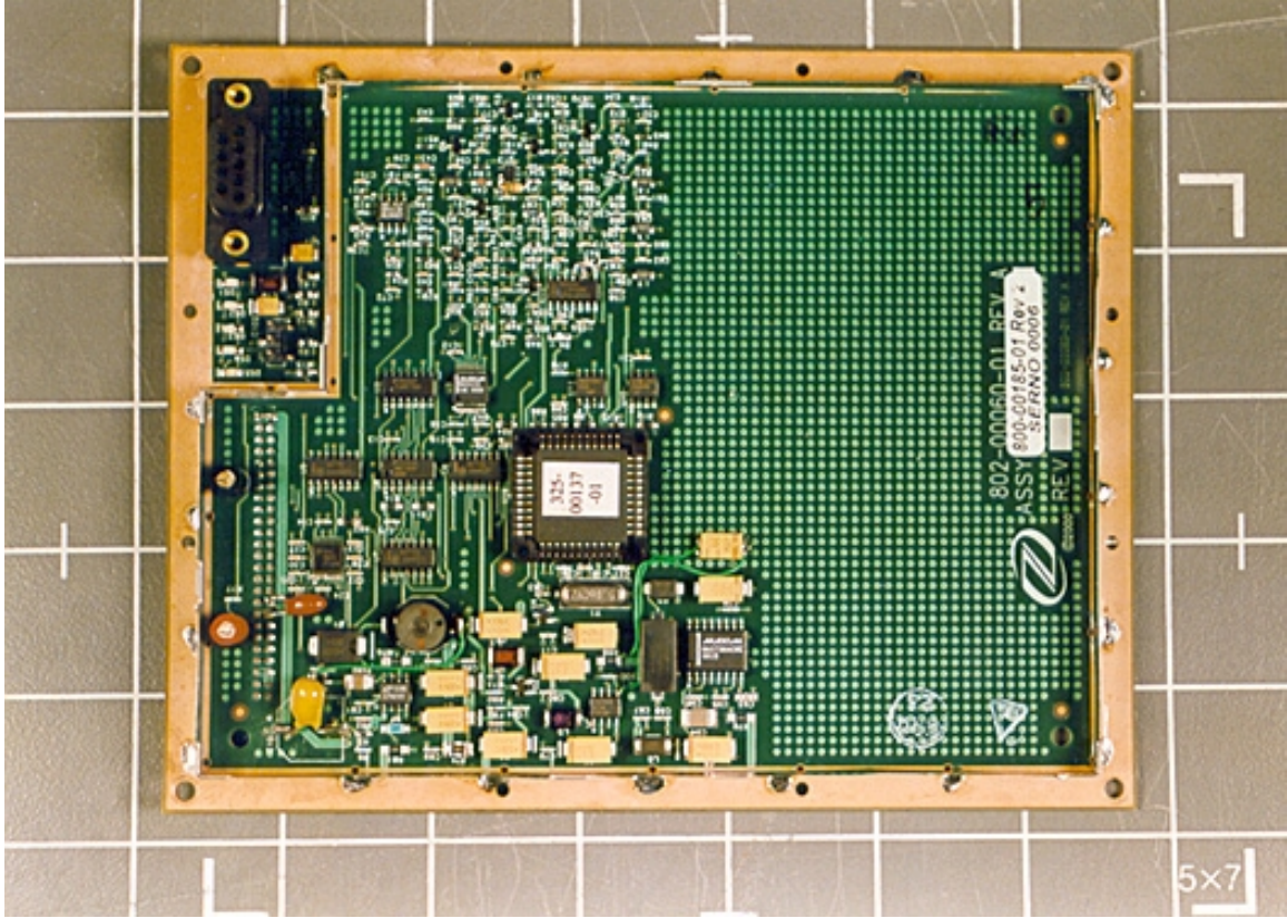
ODU B – Front PCB
