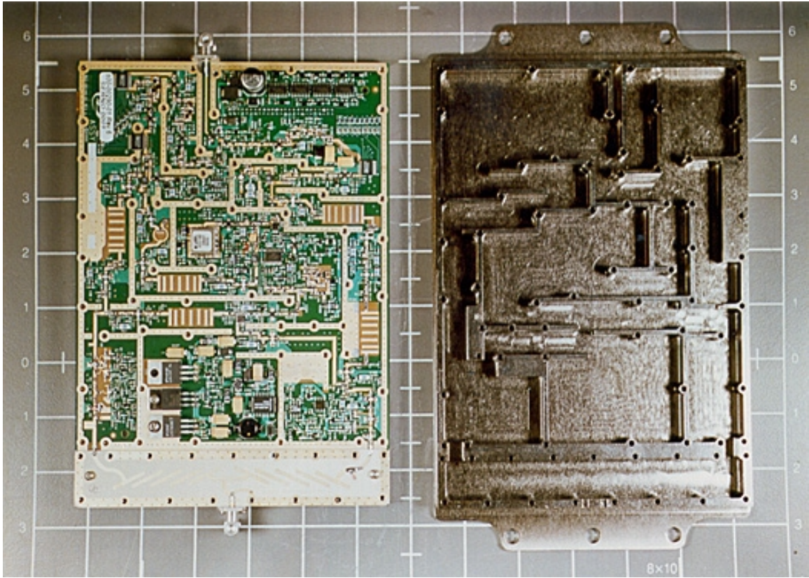
ODU B – Back PCB With Enclosure Split
