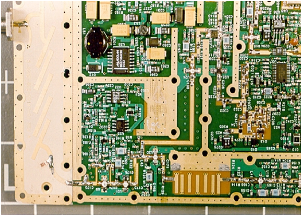
ODU B – Back PCB, Quarter View
