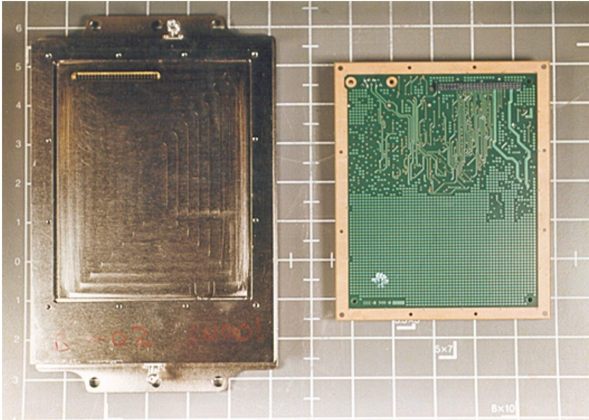
ODU B – Front With Front PCB Split
