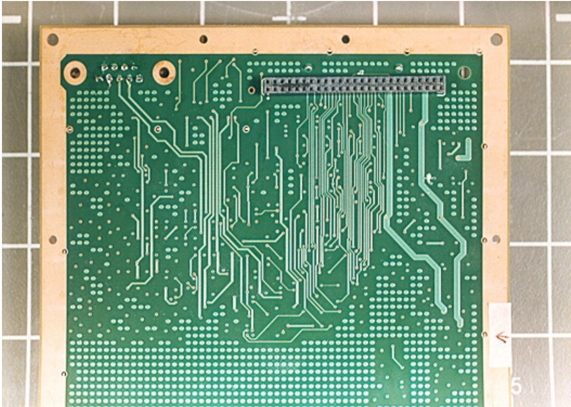
ODU B – Front PCB, Back Right
