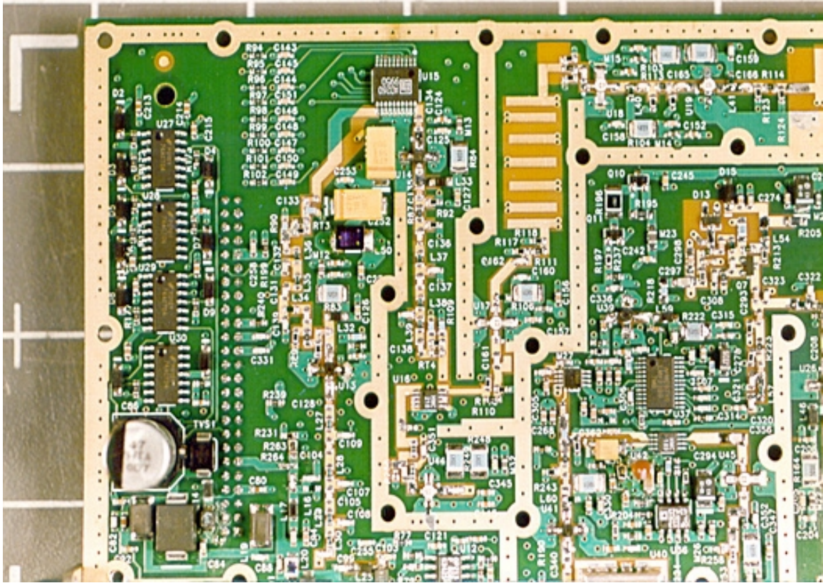
ODU B – Back PCB, Quarter View
