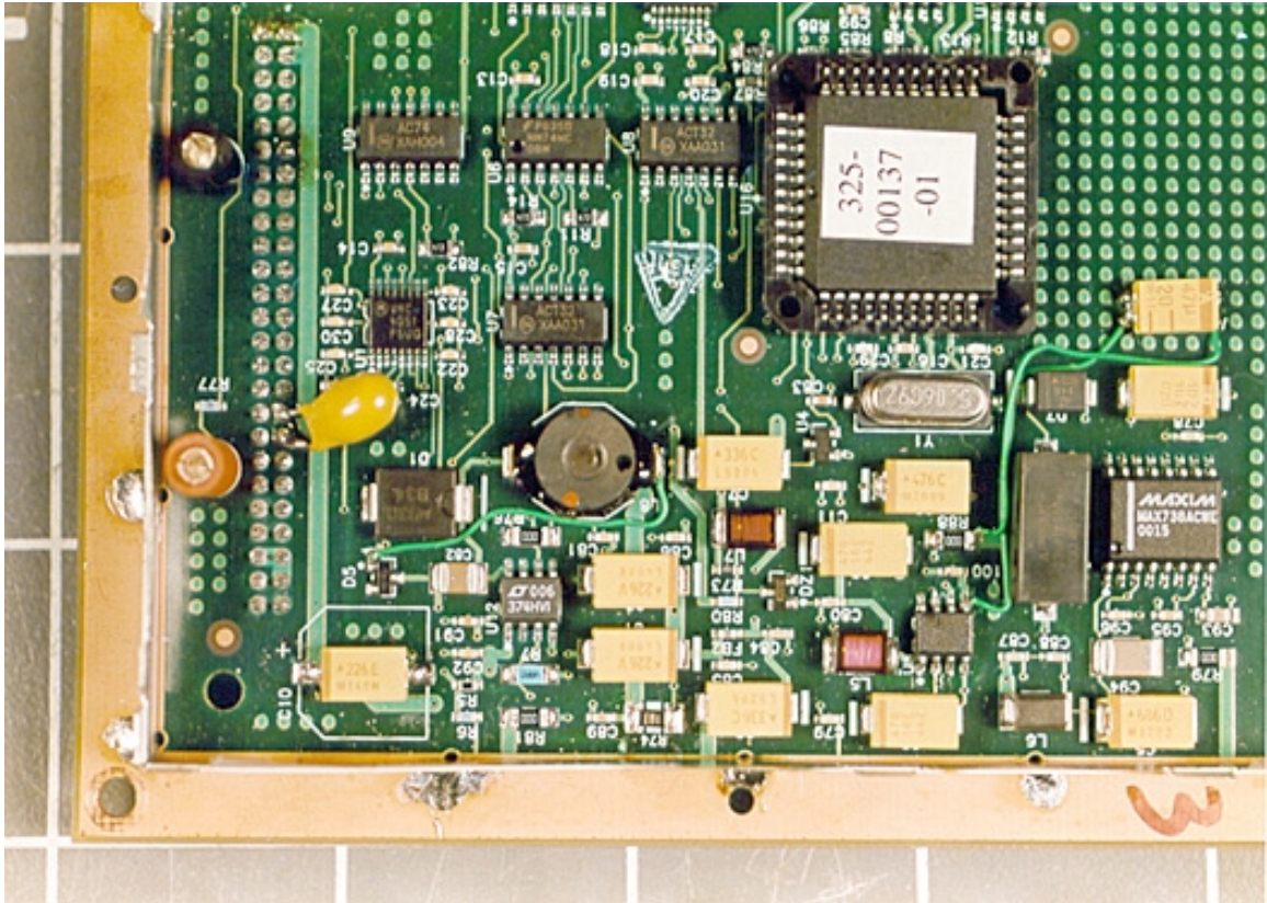
ODU B – Front PCB, in Thirds
