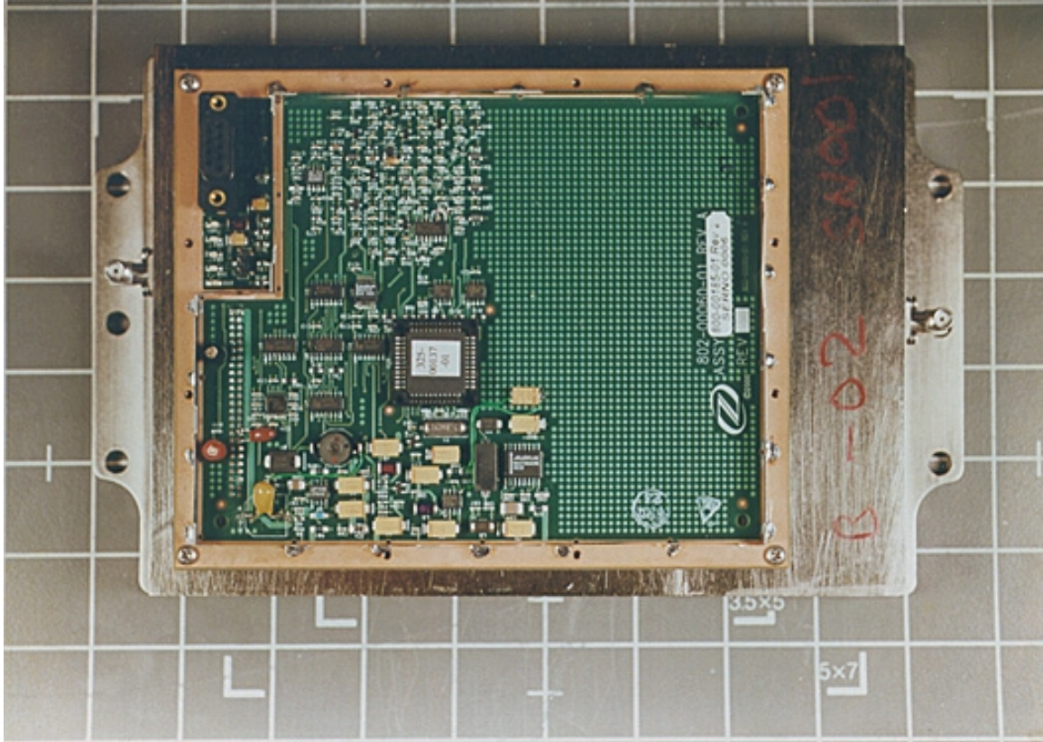
ODU B – Inside Front Without Shield
