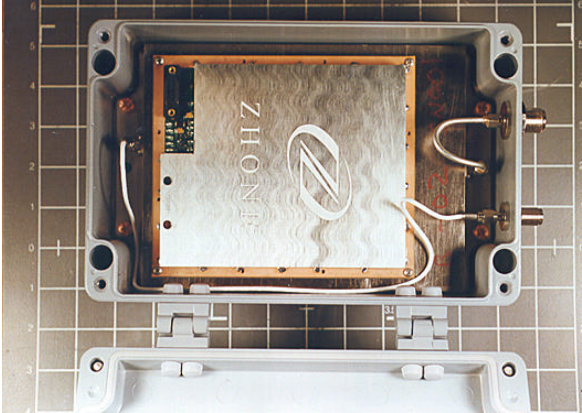
ODU B – Inside Front
