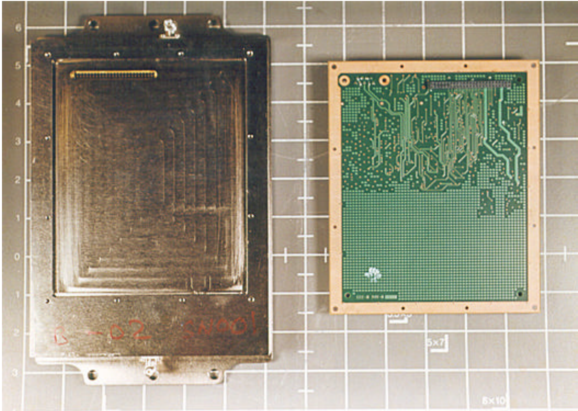
ODU B – Front With Front PCB Split
