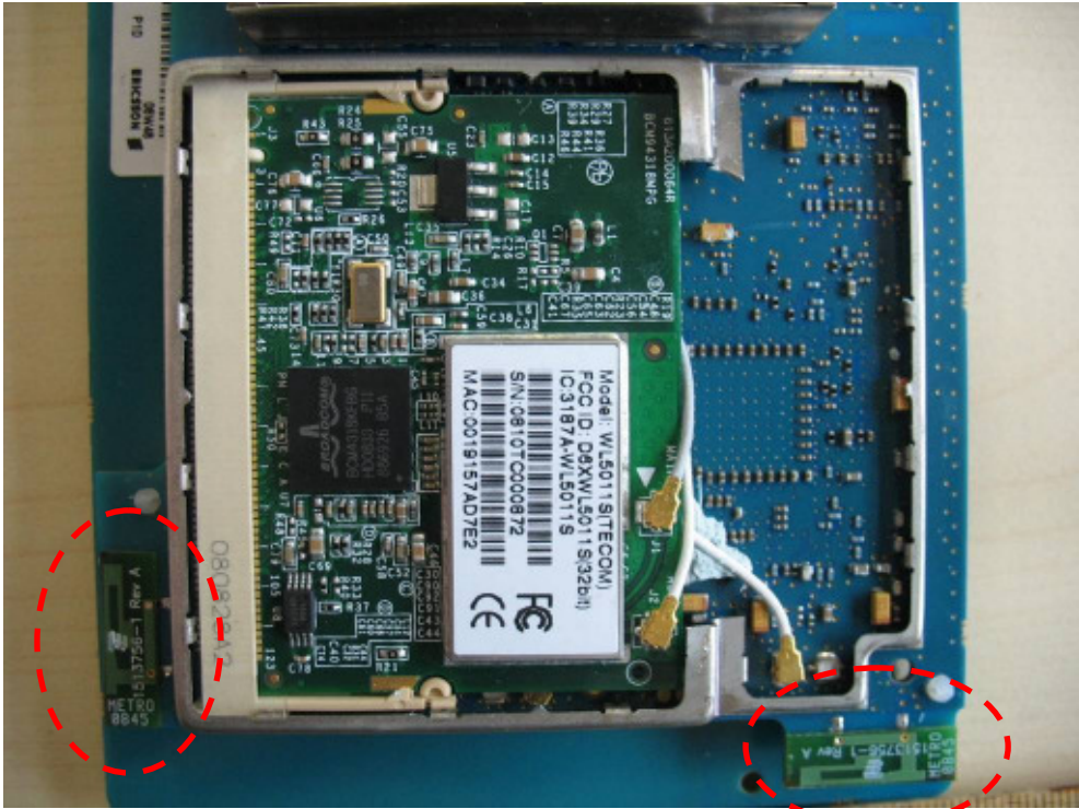
Photo 25: (WLAN-Antenna)
