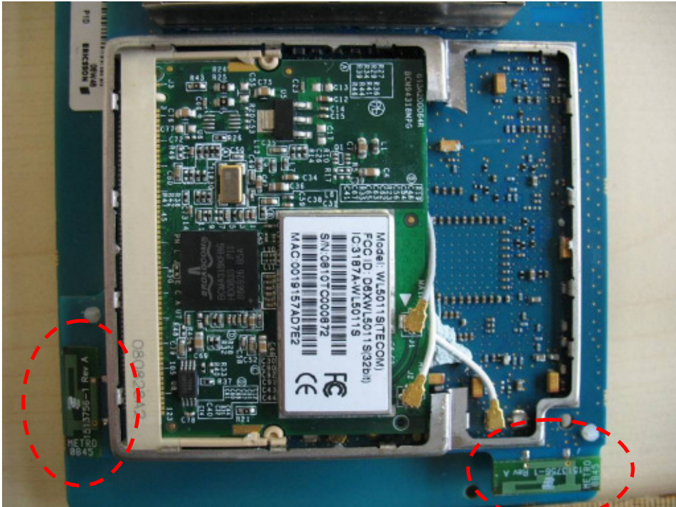
Photo 25: (WLAN-Antenna)
