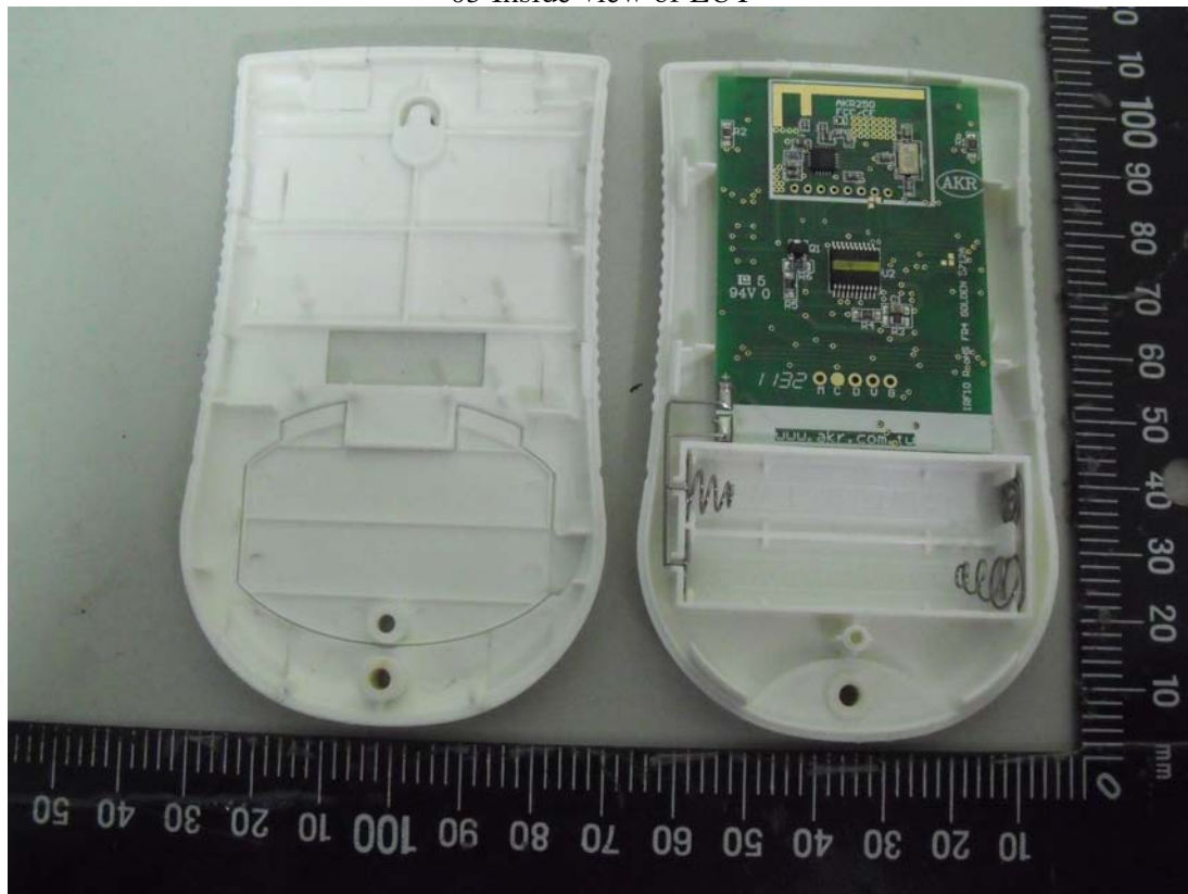
03 Inside view of EUT
