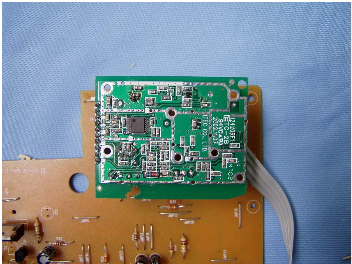
Internal Photograph of Handset Unit
