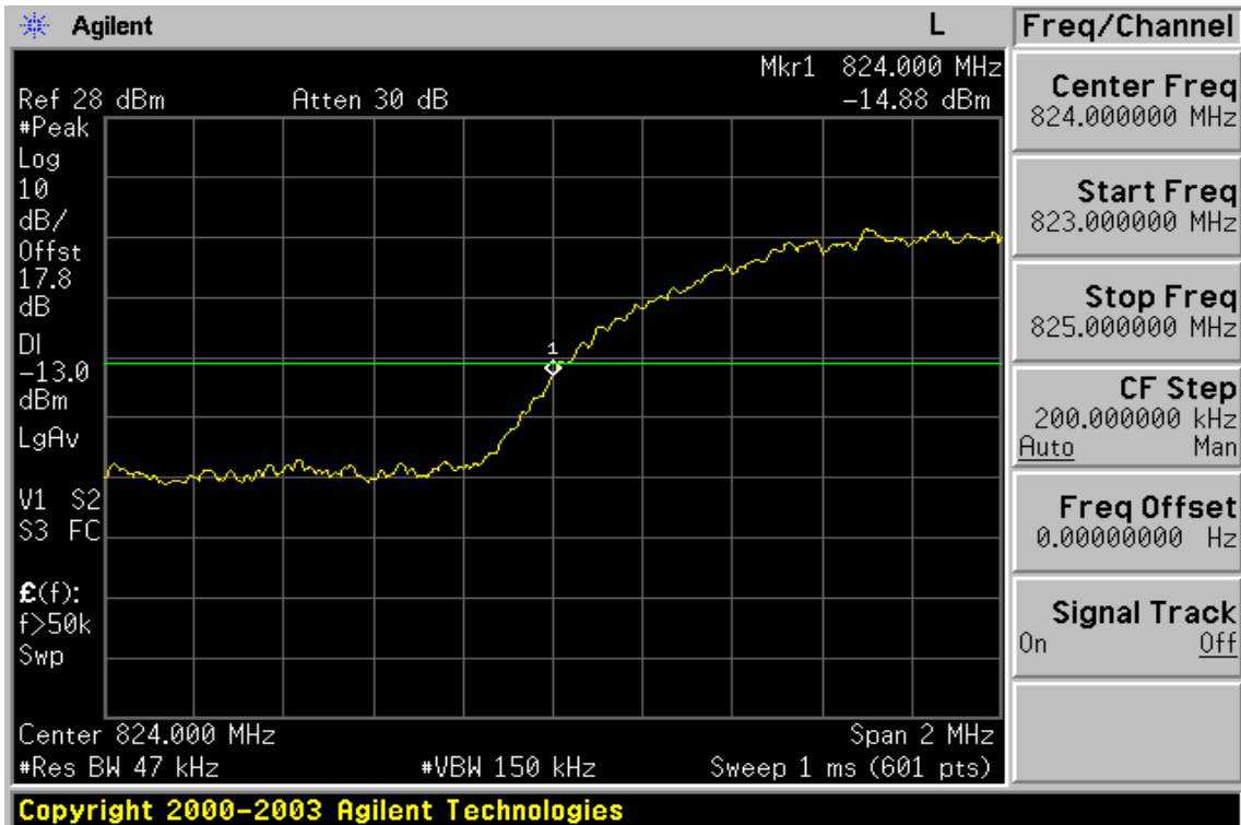
Figure 8-17: Band edge emission at antenna terminals – WCDMA BAND V Channel Lowest
