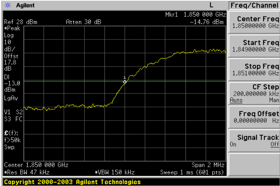
Figure 8-13: Band edge emission at antenna terminals – WCDMA BAND II Channel Lowest
