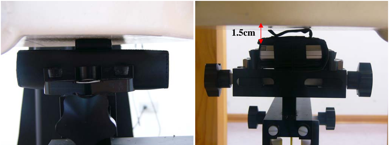
Fig.8 Body worn- EUT back to flat phantom (testing in GPRS Mode)
