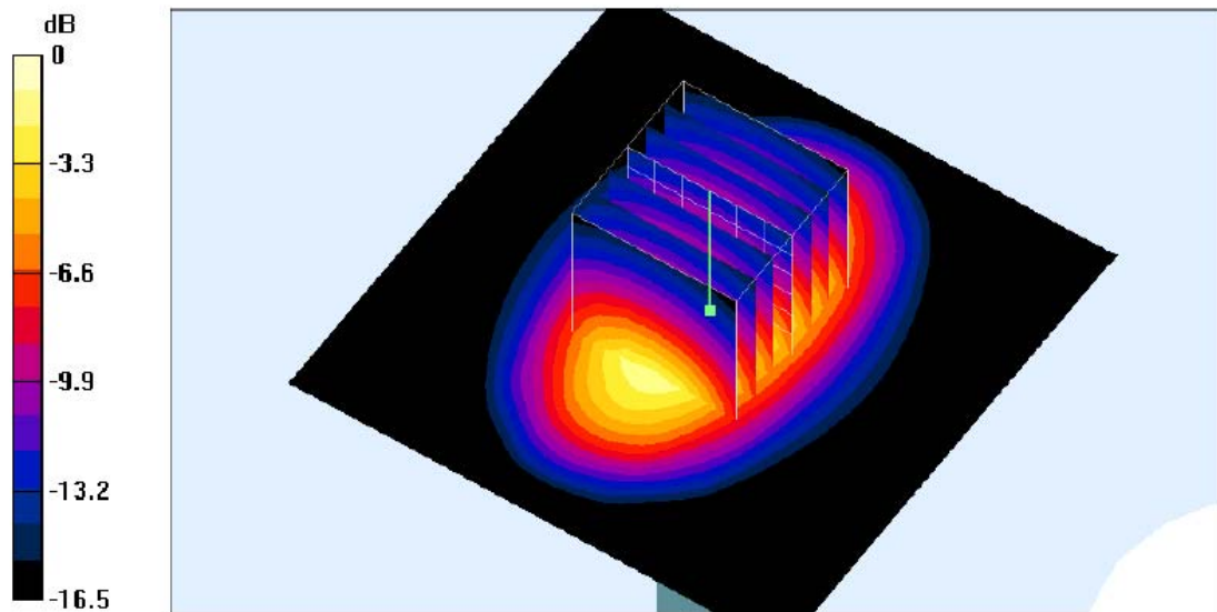
0 dB = 4.49mW/g
