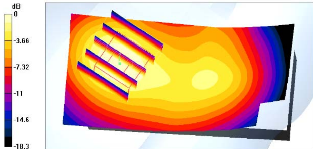
0 dB = 0.648mW/g
