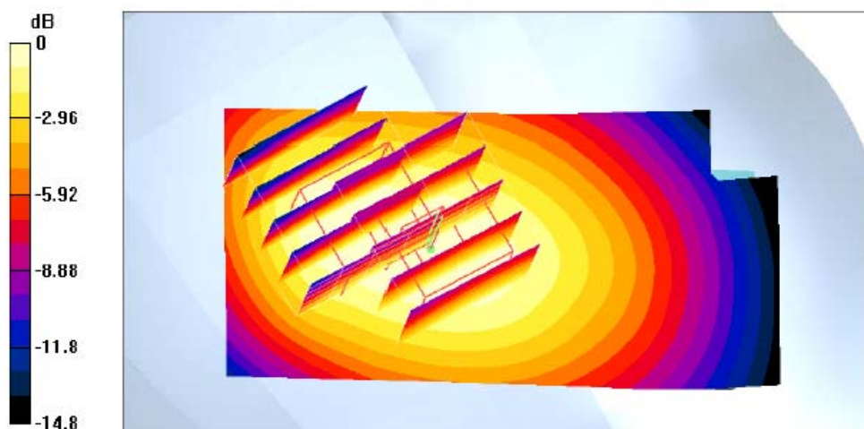
0 dB = 0.651mW/g
