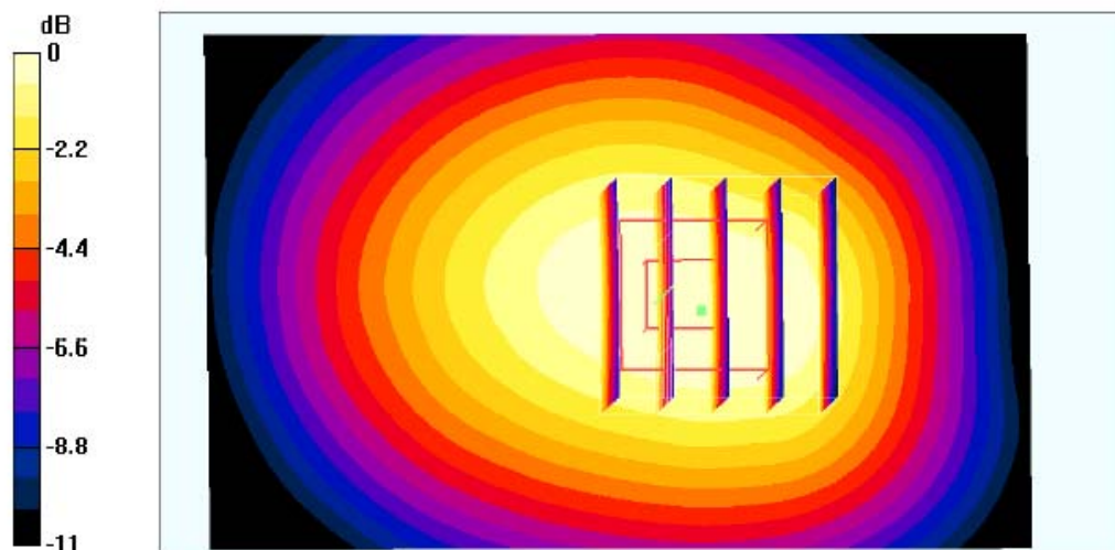
0 dB = 0.718mW/g
