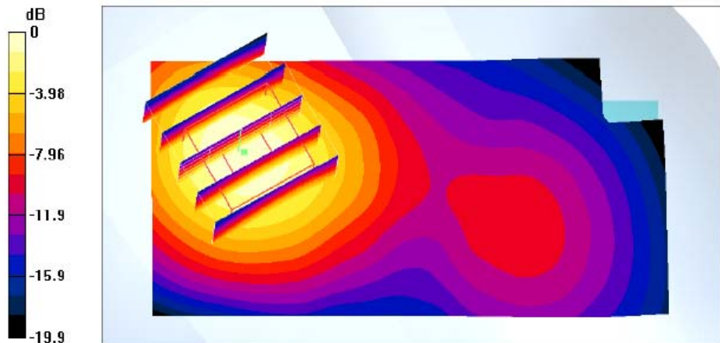
0 dB = 0.873mW/g
