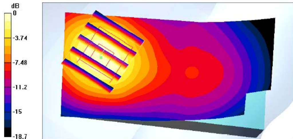
0 dB = 0.704mW/g
