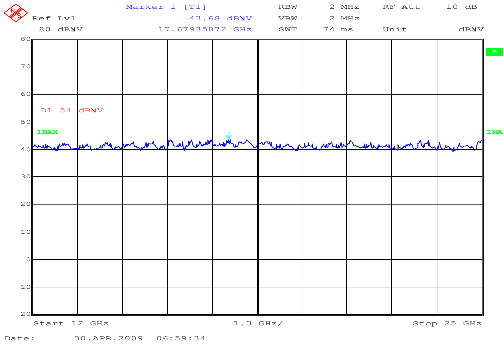
Plot 6: 12GHz – 25 GHz (h/v worst case) valid for all channels
