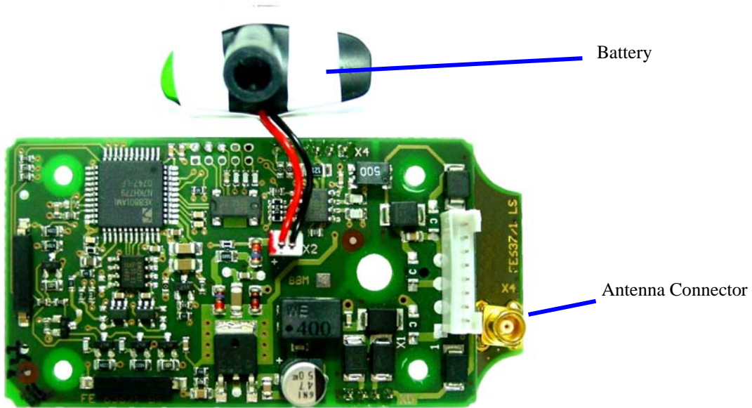
Component Side FE636/1 (Positioning Encoder) and parts of Radio Board FE637/1 Solder Side
