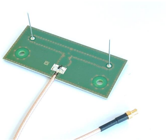
Fig. 6: Internal view on bottom side of TST PD2_FSAS-C antenna
