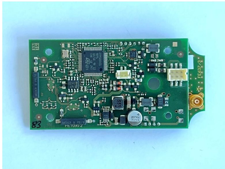
Fig. 3: View on PCBs of Stationary Wireless Unit FSAS-C (FE637/3, behind Encoder PCB FE1090/2)
