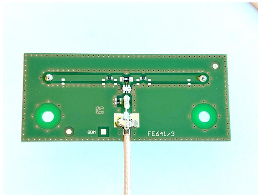
Fig. 7: Internal view on top side of TST PD2_FSAS-C antenna
