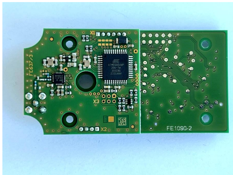
Fig. 4: Bottom view of Stationary Wireless Unit FSAS-C (FE637/3)
