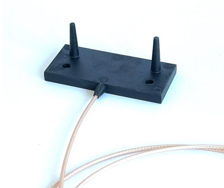
Fig. 2: External view of TST PD2_FSAS-C antenna
