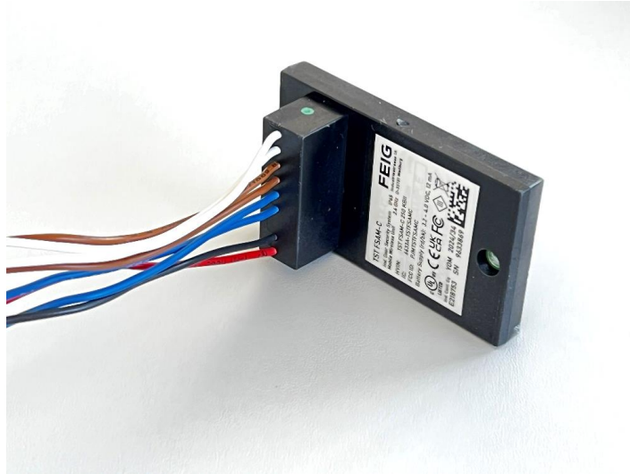
Fig. 1: External view onto Mobile Wireless Unit FSAM-C from connecting wires side
