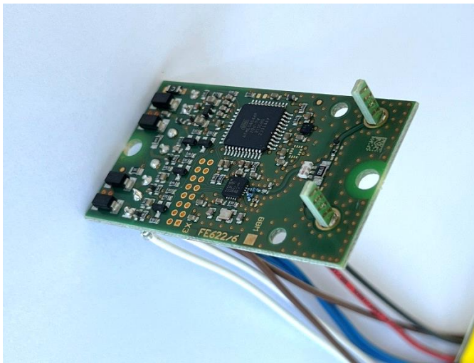
Fig. 4: Internal view onto Mobile Wireless Unit FSAM-C from antennas side
