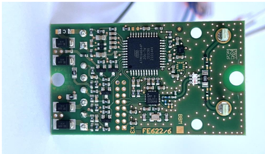
Fig. 5: Detailed internal view onto Mobile Wireless Unit FSAM-C
