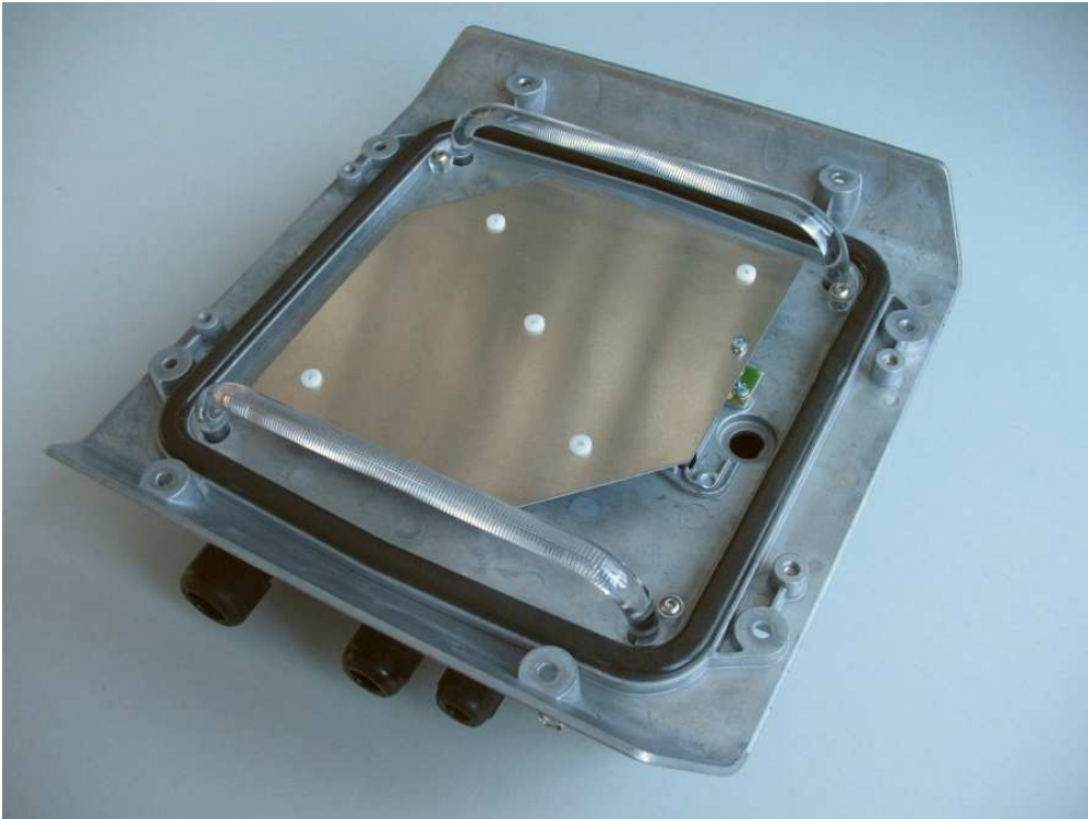
Image 2, front cover removed, viewing antenna and light guides:
