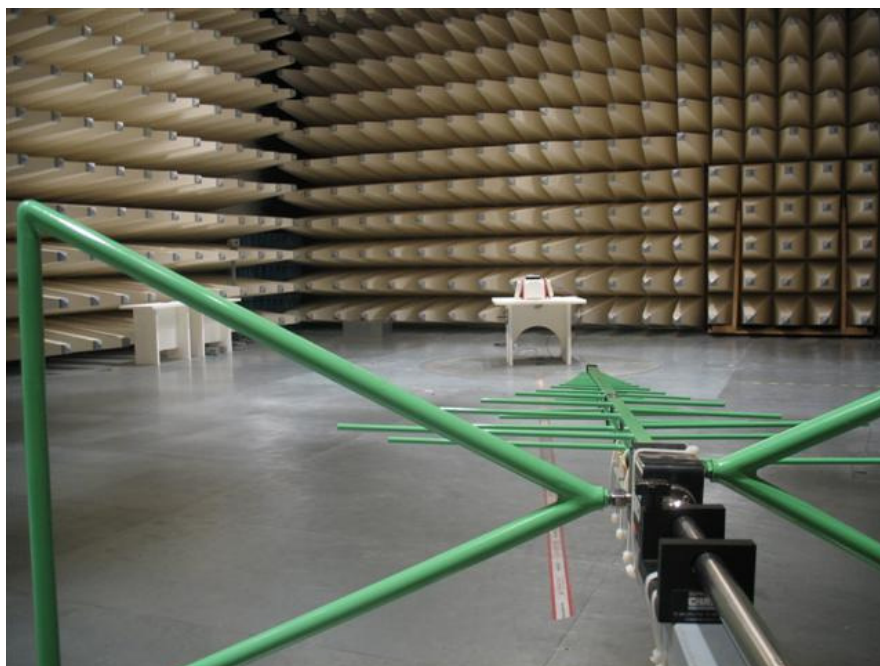
Photo 2: Radiated Emissions
