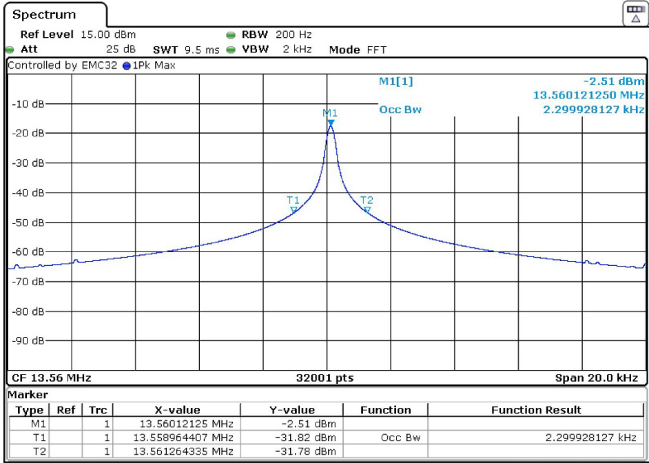
99% Bandwidth
