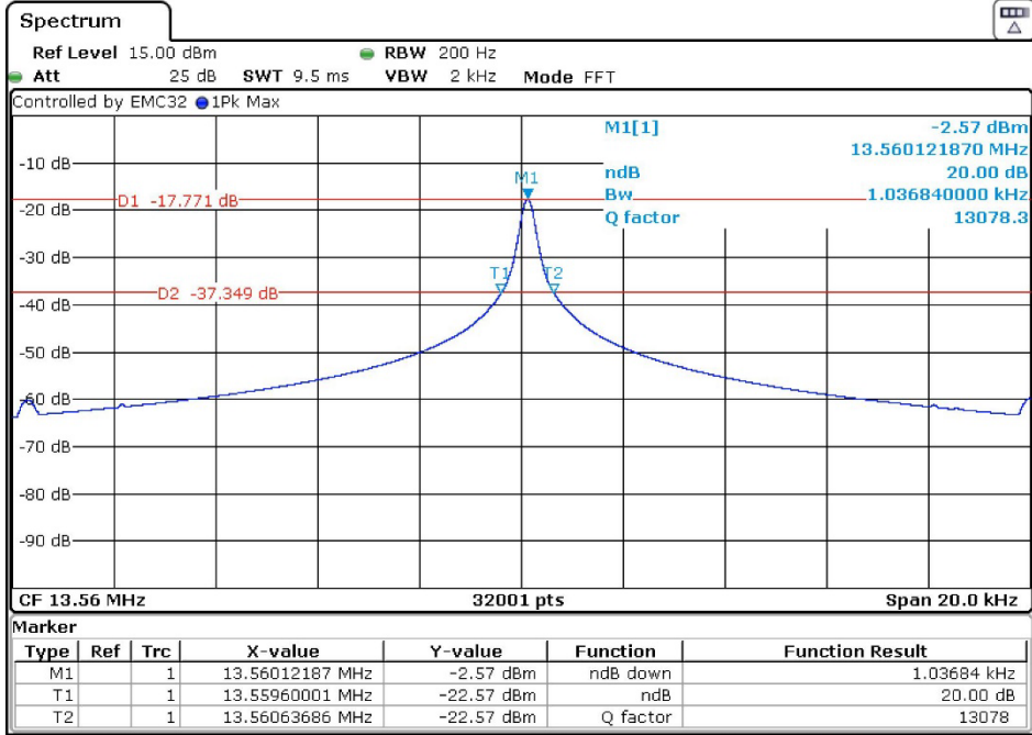
20 dB Bandwidth
