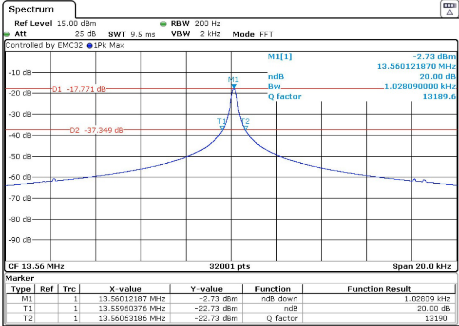
20 dB Bandwidth
