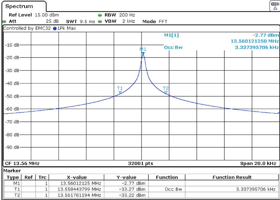
99% Bandwidth
