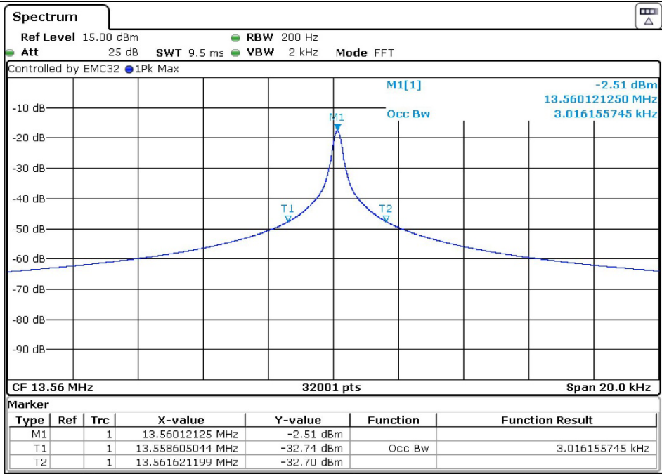
99% Bandwidth
