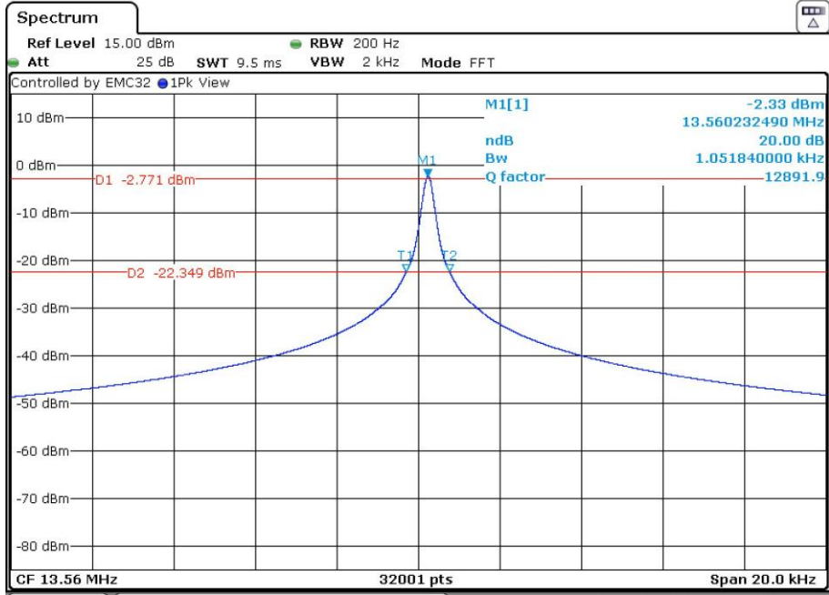
20 dB Bandwidth
