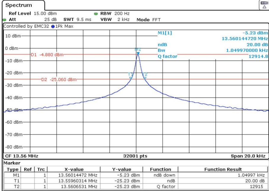
20 dB Bandwidth
