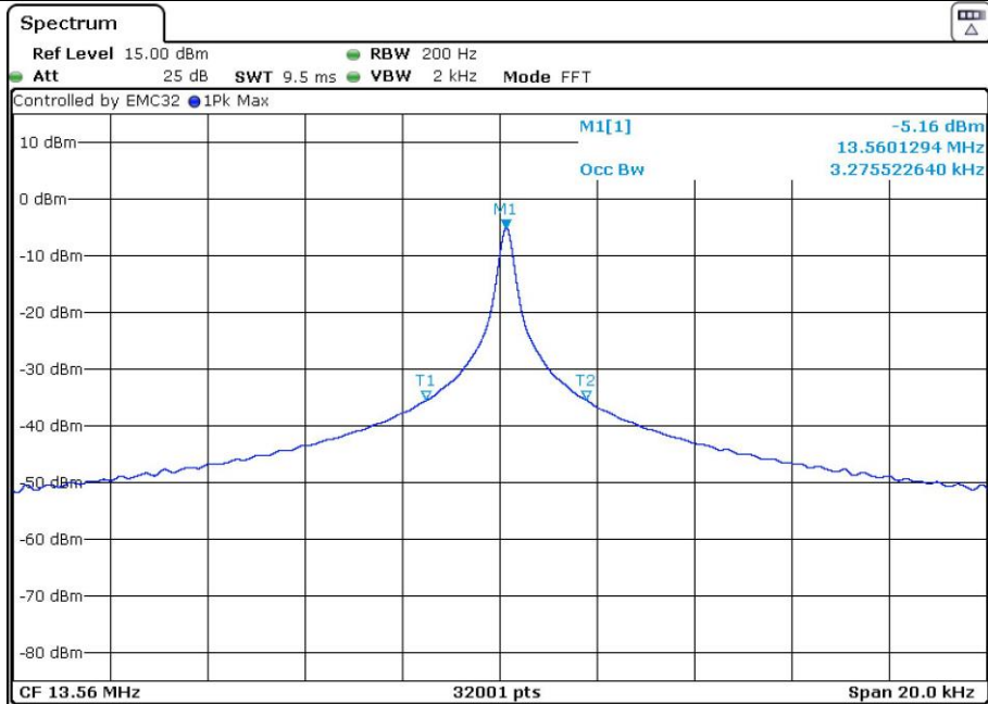
99% Bandwidth
