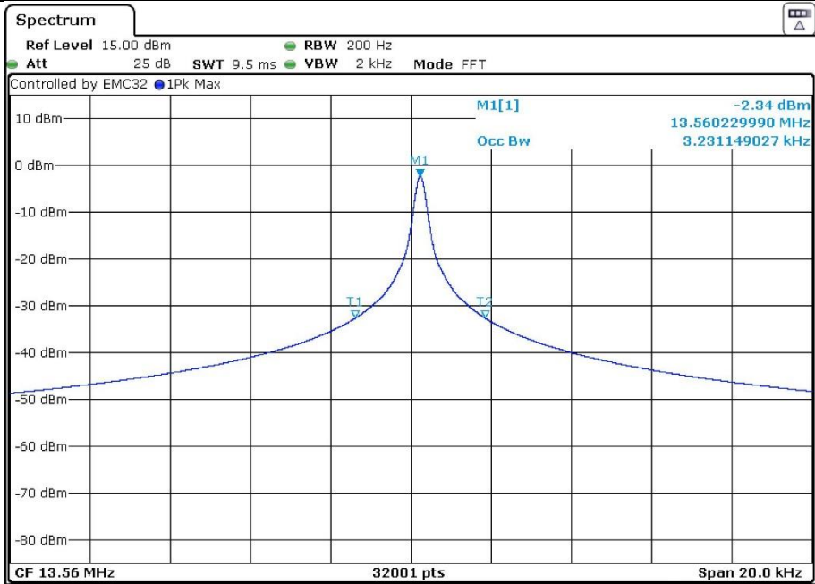
99% Bandwidth
