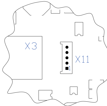
Figure 15: USB-Interface for host communication
