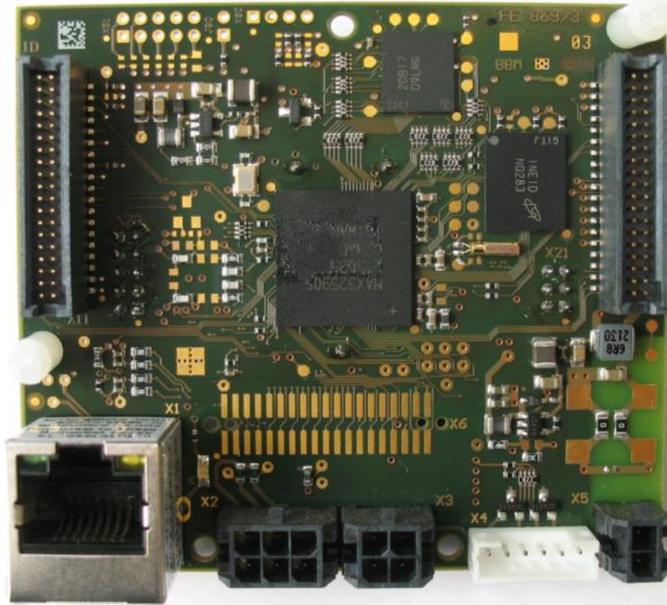
Core PCB top
