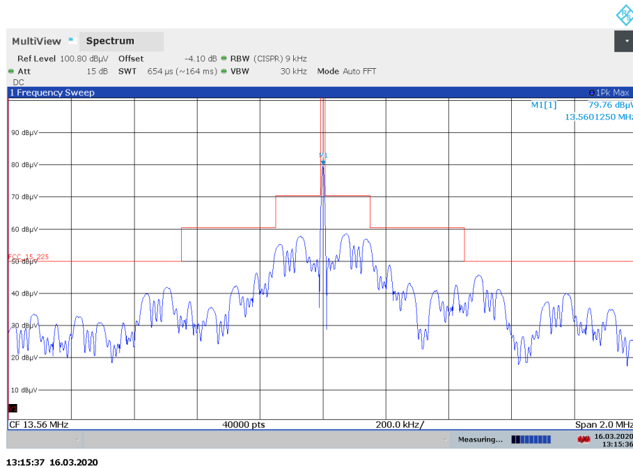
Plot 2: Spectrum mask peak (worst case, the limits are re-calculated according to the ANSI C63.10-2013 sub clause 6.4)
